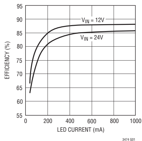
Efficiency, Two LED Output
