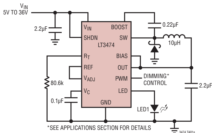
Step-Down 1A LED Driver
