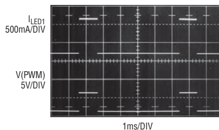
LED Current in PWM Mode
