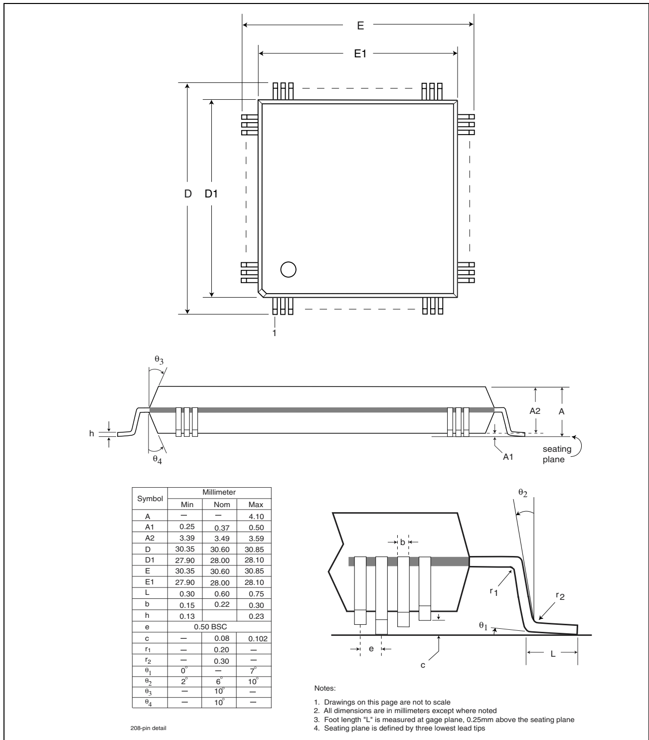
Figure 11: 208-Pin PQFP
