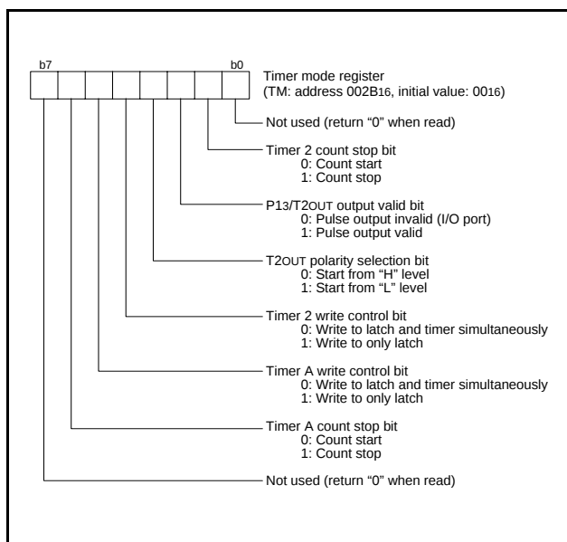
Fig 26. Structure of timer mode register
