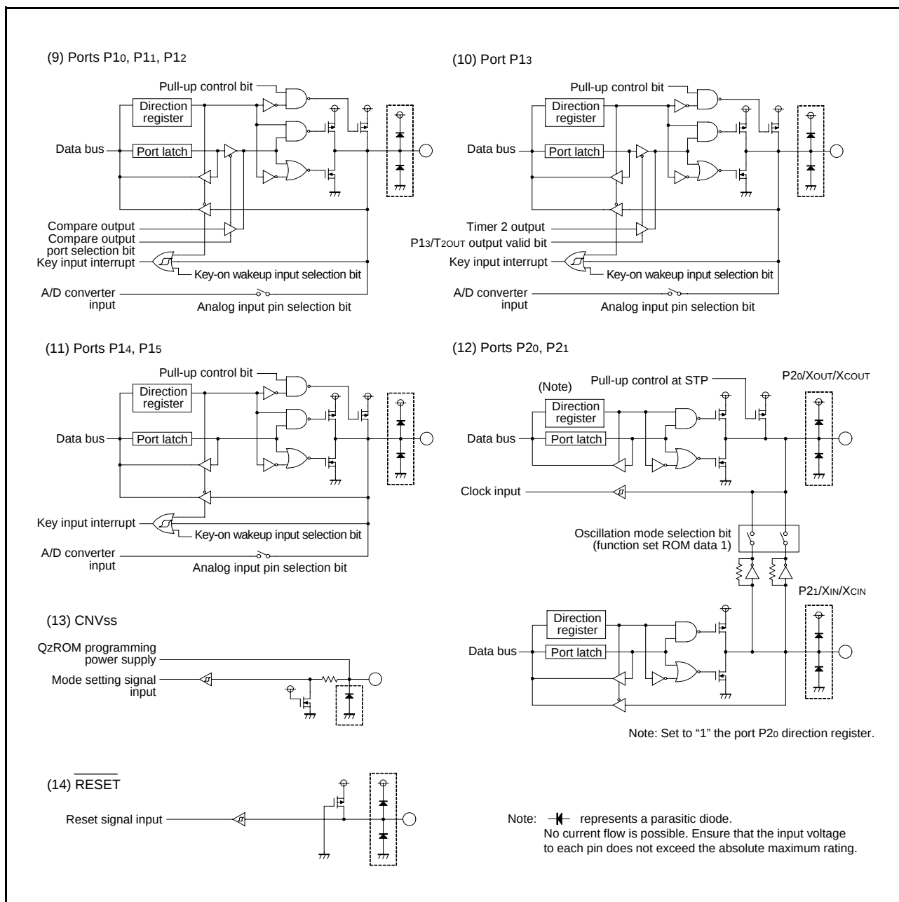
Fig 18. Block diagram of pins (2)
