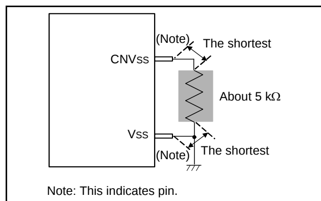
Fig 76. Wiring for the VPP pin of the QzROM
