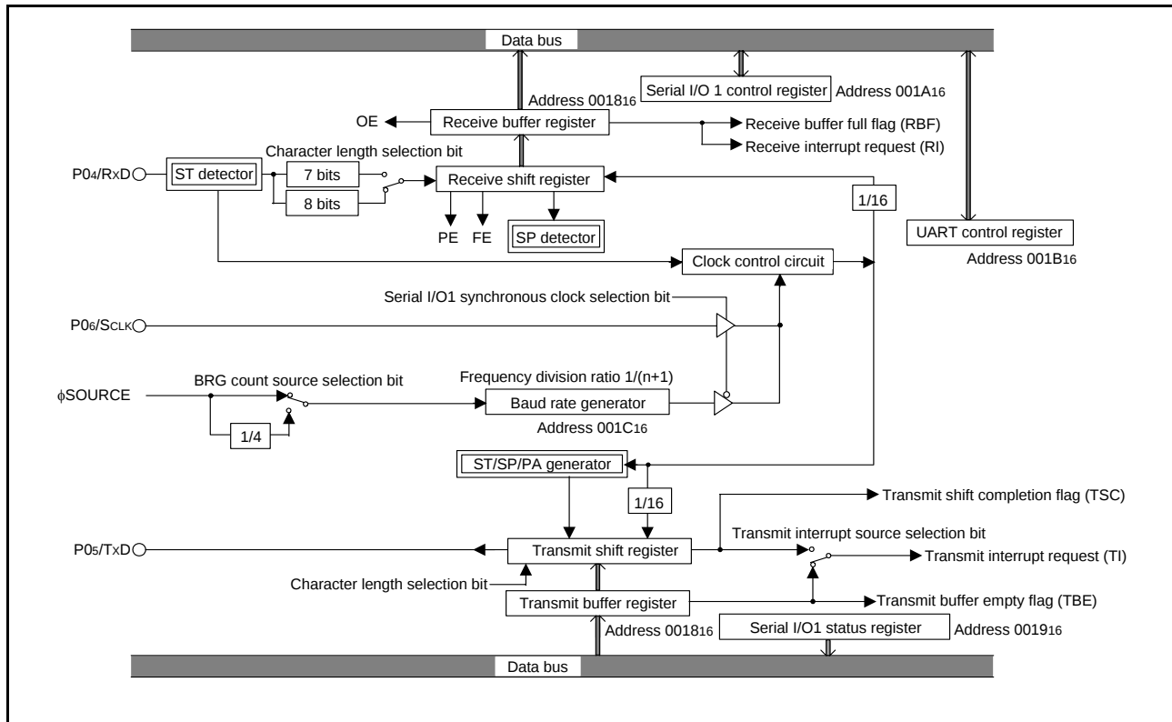
Fig 48. Block diagram of UART serial I/O
