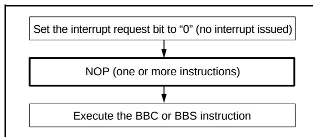
Fig 91. Sequence of check of interrupt request bit
