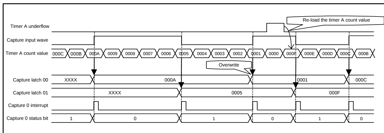
Fig 45. Capture input waveform (capture interrupt edge selection bit = "rising and falling edge")
