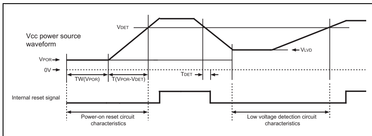
Fig 84. Electrical characteristics of power-on reset circuit and low voltage detection circuit
