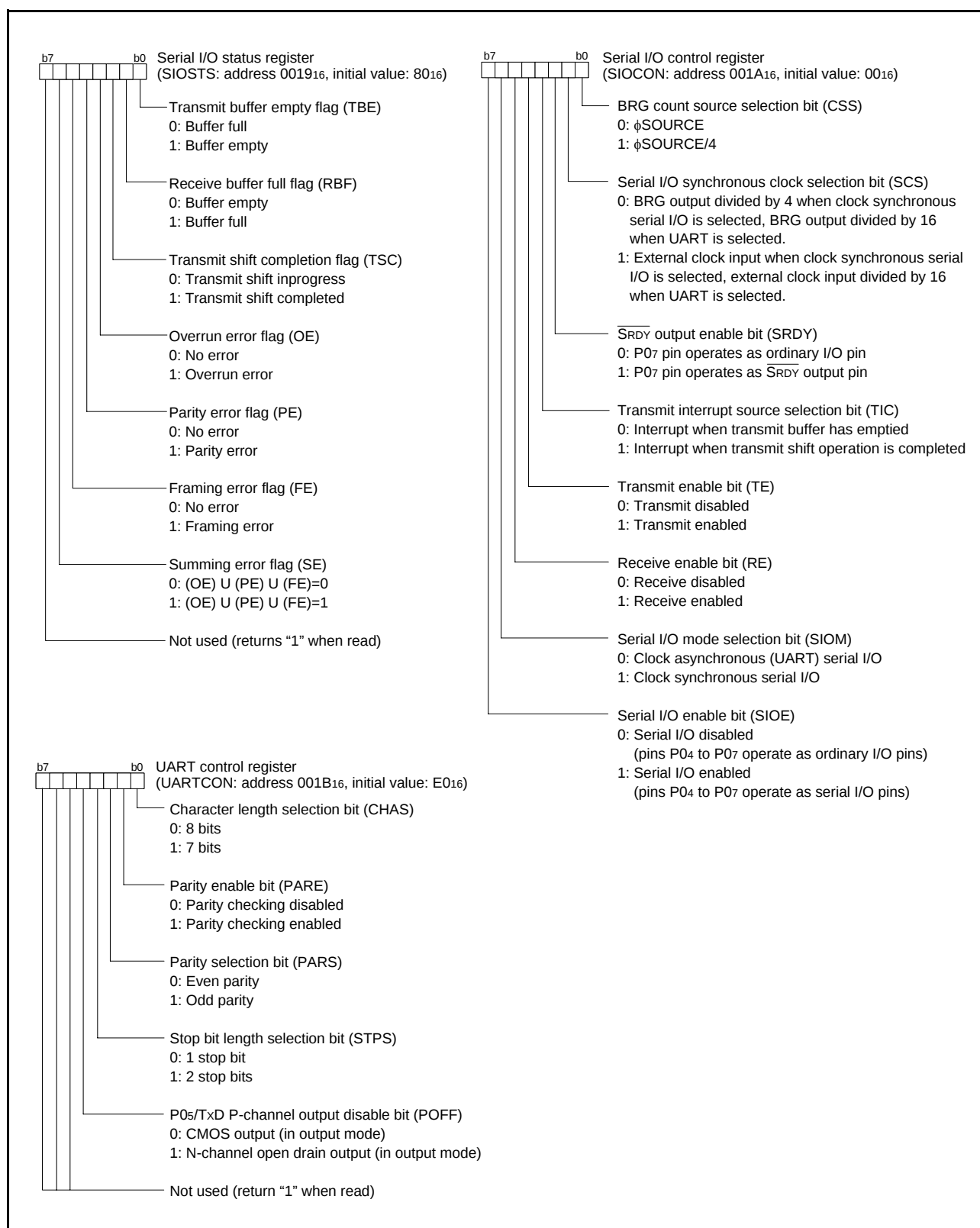
Fig 50. Structure of serial I/O1-related registers
