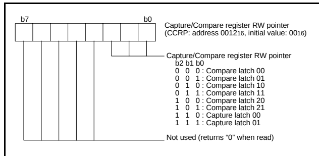
Fig 31. Structure of capture/compare register RW pointer
