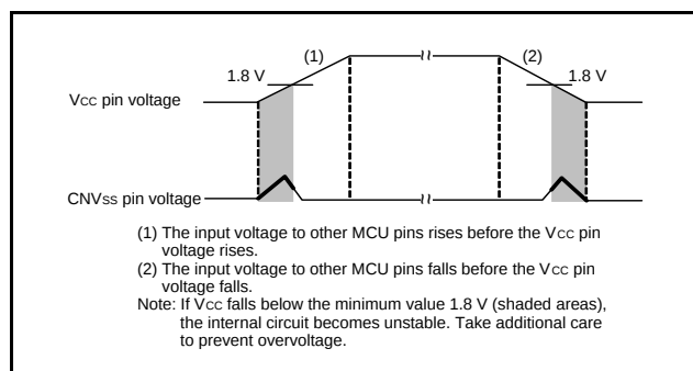
Fig 92. Timing Diagram (bold-lined periods are applicable)
