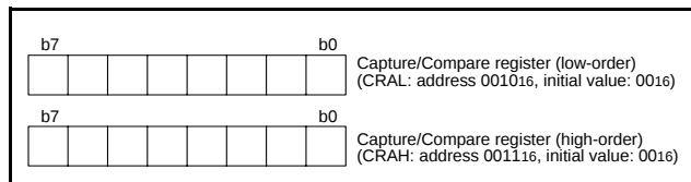
Fig 30. Structure of capture/compare register
