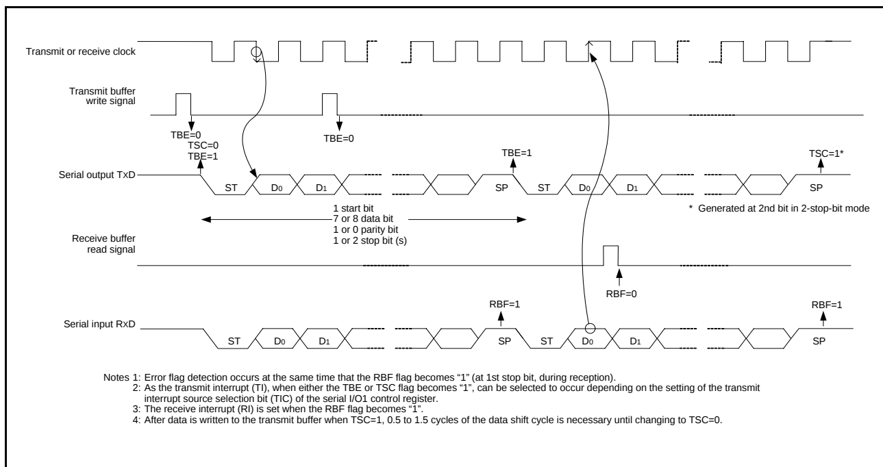
Fig 49. Operation of UART serial I/O function
