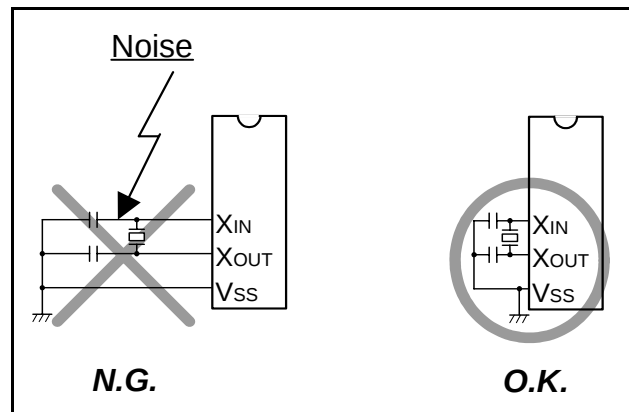
Fig 75. Wiring for clock I/O pins
