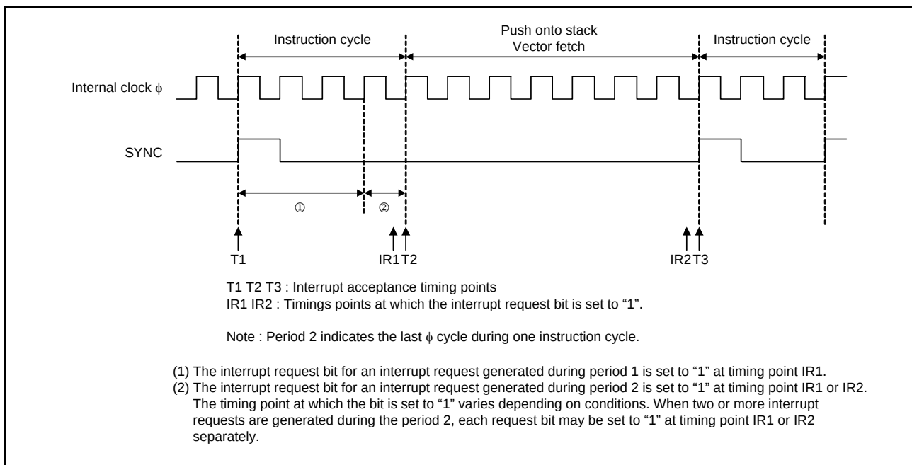
Fig 23. Timing of interrupt request generation, interrupt request bit, and interrupt acceptance
