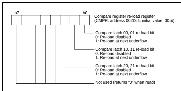
Fig 32. Structure of compare register re-load register
