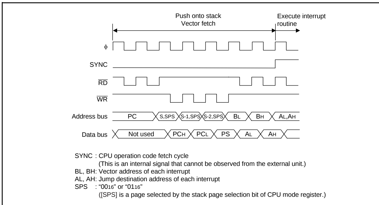
Fig 22. Interrupt sequence
