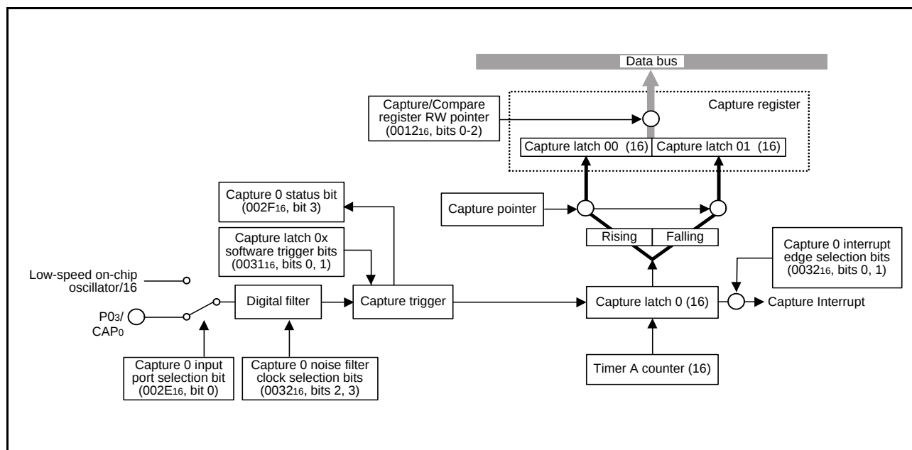
Fig 43. Block diagram of capture channel 0
