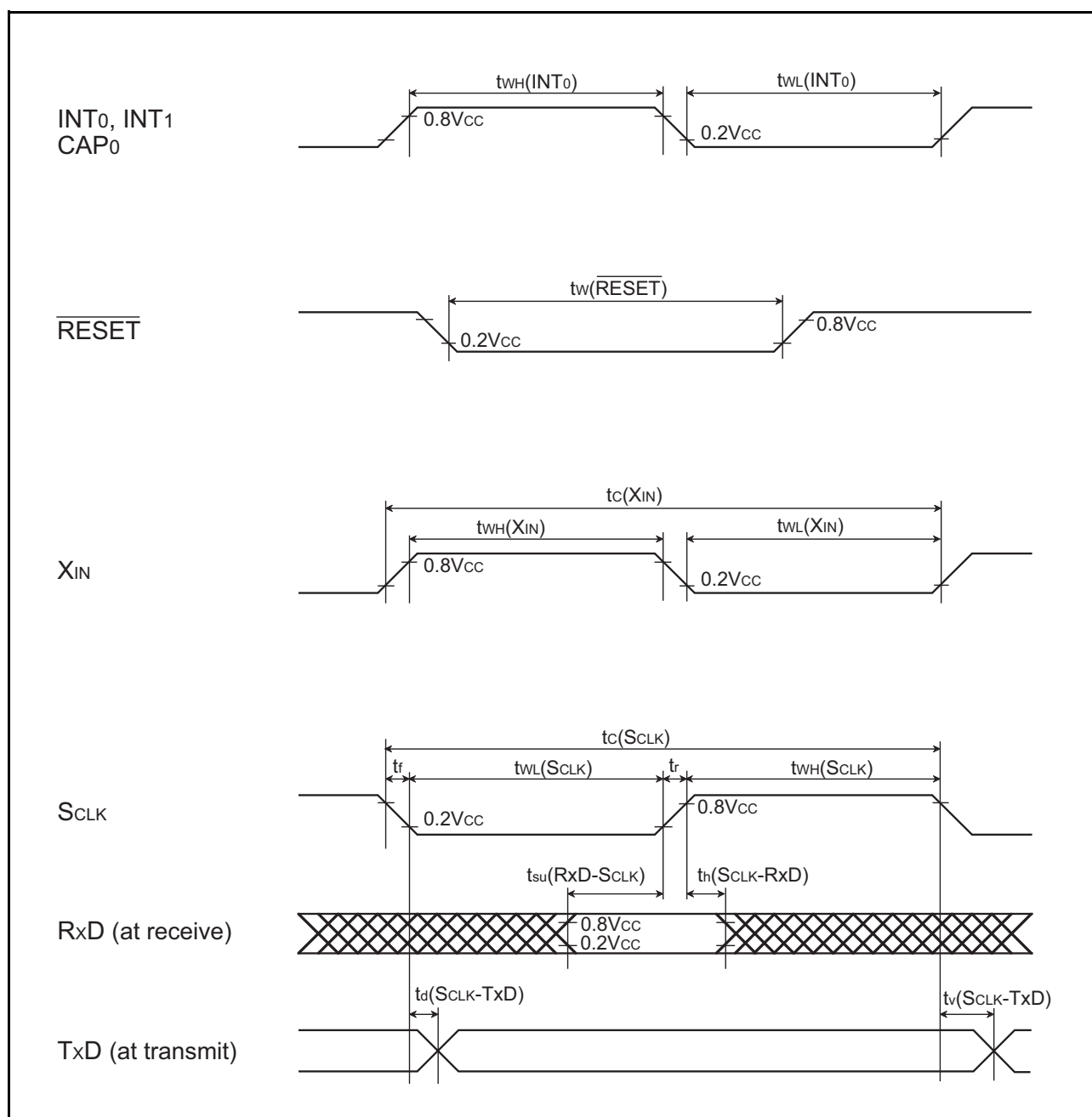
Fig 86. Timing chart
