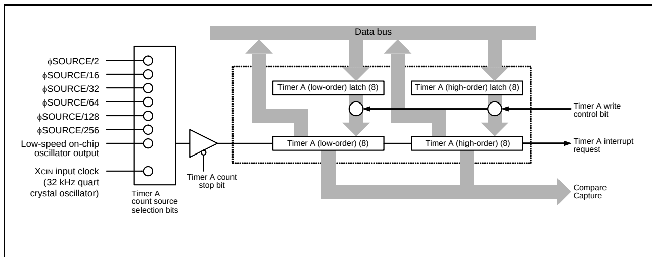
Fig 29. Block diagram of timer A
