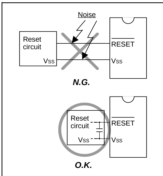
Fig 74. Wiring for the RESET pin
