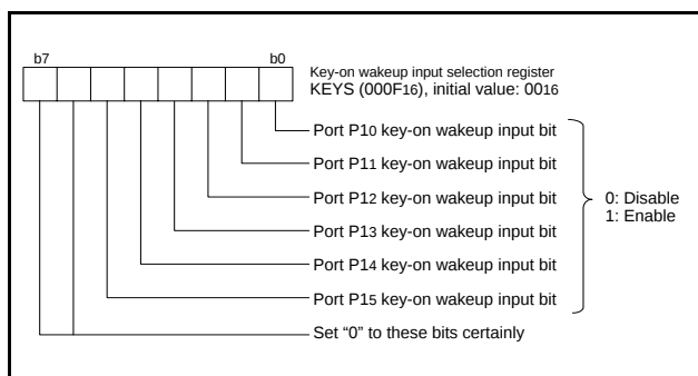
Fig 25. Structure of key input control register
