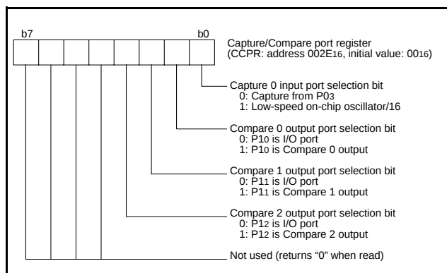
Fig 33. Structure of capture/compare port register
