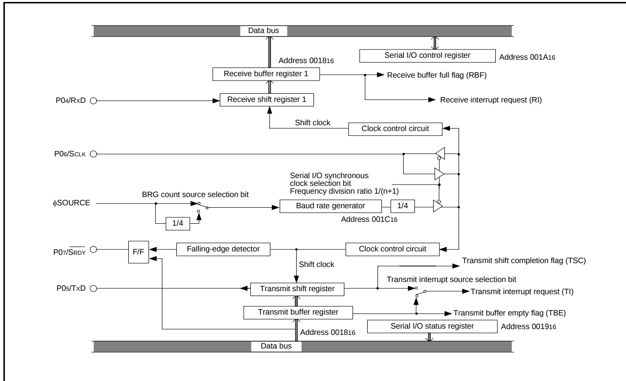
Fig 46. Block diagram of clock synchronous serial I/O
