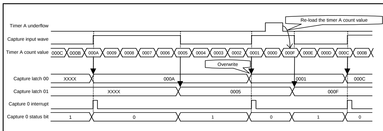
Fig 44. Capture input waveform (capture interrupt edge selection bit = "rising edge")
