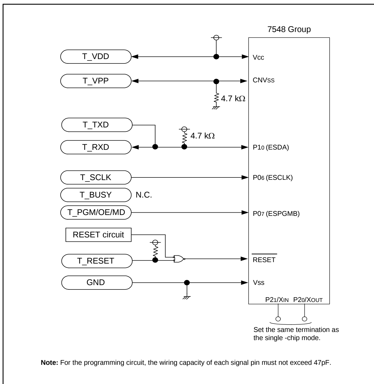
Fig 72. When using programmer of Suissei Electronics System Co., LTD, connection example
