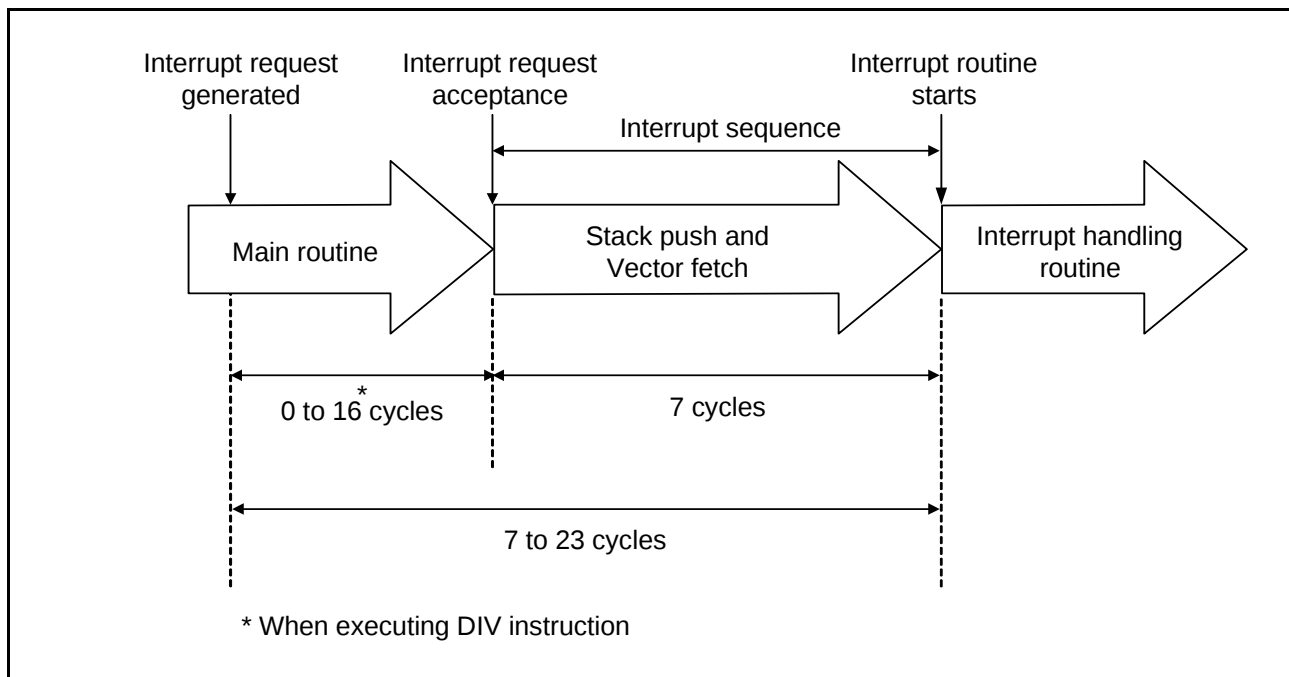
Fig 21. Time up to execution in interrupt routine
