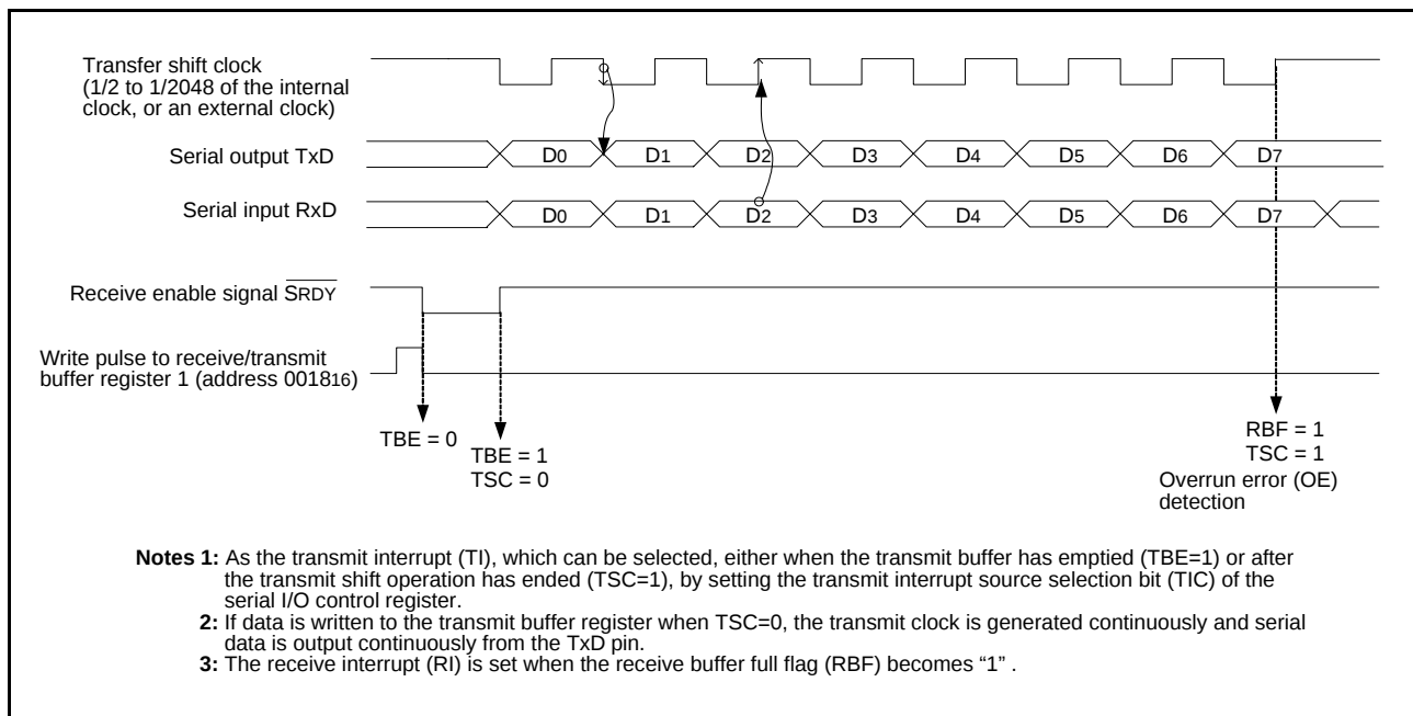
Fig 47. Operation of clock synchronous serial I/O function
