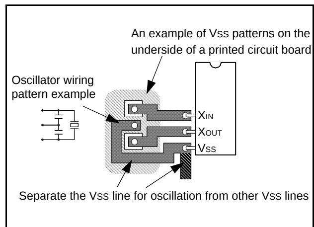
Fig 79. Vss pattern on the underside of an oscillator
