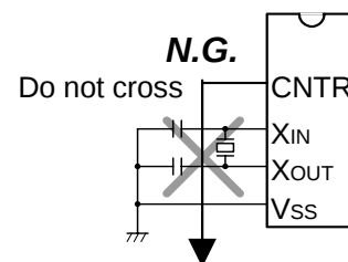
Fig 78. Wiring for a large current signal line/Writing of signal lines where potential levels change frequently
