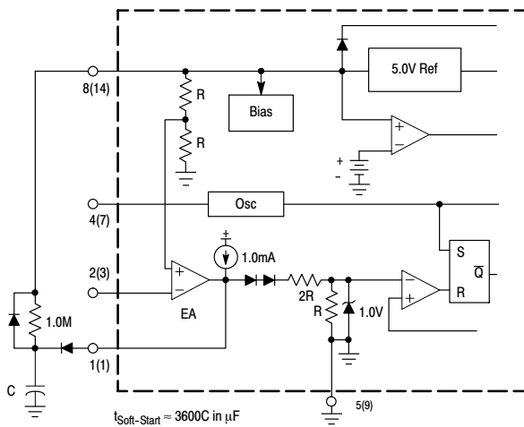
Figure 25. Soft-Start Circuit
