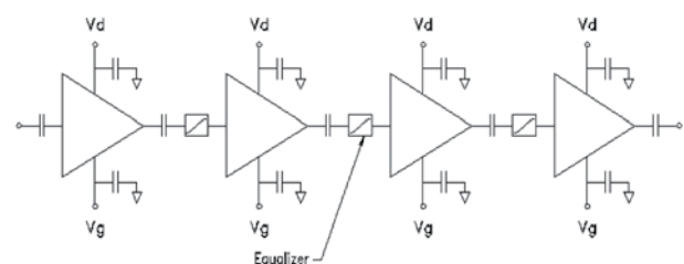
Typical Broadband Module for Fiber Optic SONET
