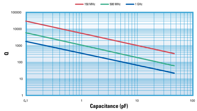
Q vs Capacitance DLI C06 CF Series
