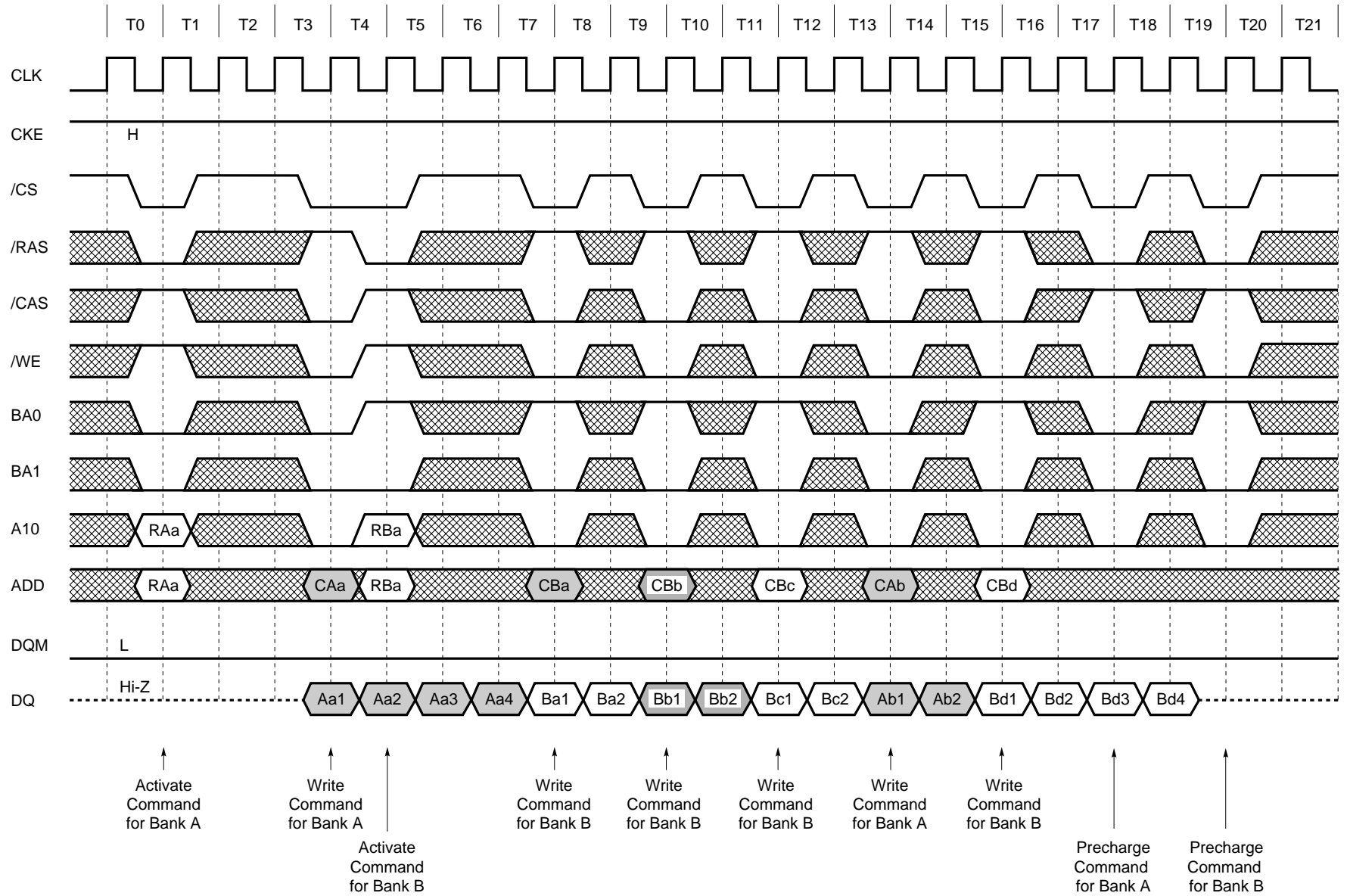
Interleaved Column Write Cycle (2/2) (Burst Length = 4, /CAS Latency = 3)
