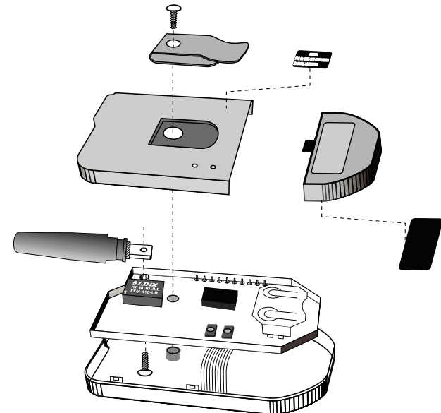
Figure 7: OTX-***-HH-LR8-MS Assembly
