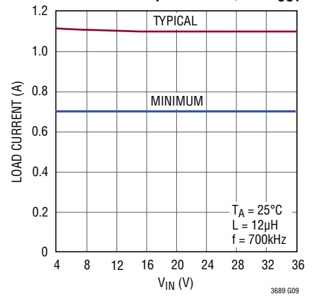
Maximum Output Current, 3.3V_{OUT}
