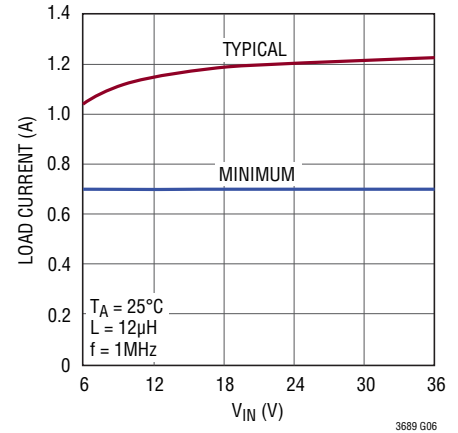
Maximum Load Current, 5V_{OUT}
