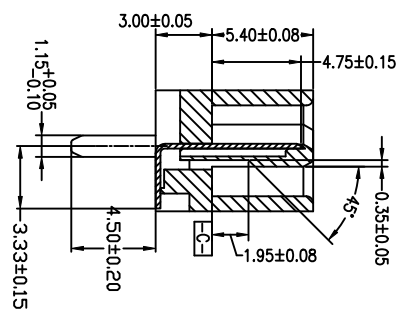
SEC. A-A Metal Clip D
