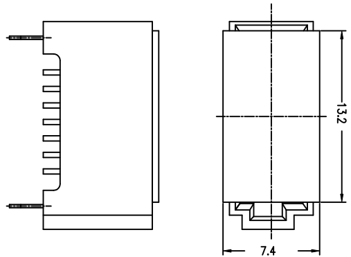
PRODUCT WITH CAP FOR T & R PACKING
