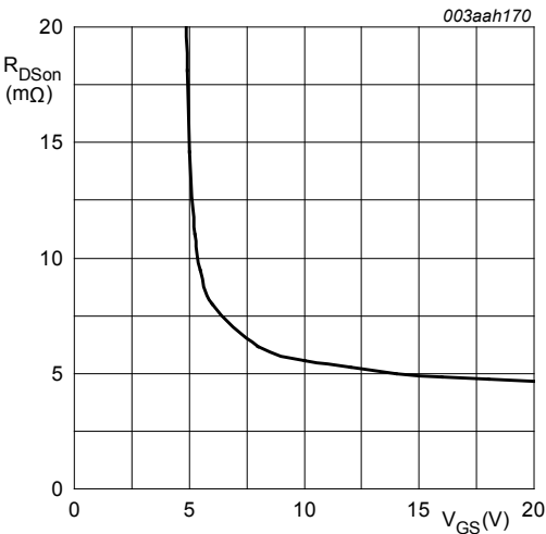
Fig. 7. Drain-source on-state resistance as a function of gate-source voltage; typical values T_j = 25\text{ °C}; I_D = 20\text{ A}
