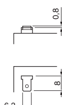
■ Type 2 Faston 6.3
