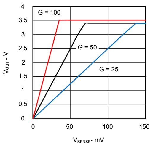
V_{OUT} vs V_{SENSE} @ Supply = 3.6V
