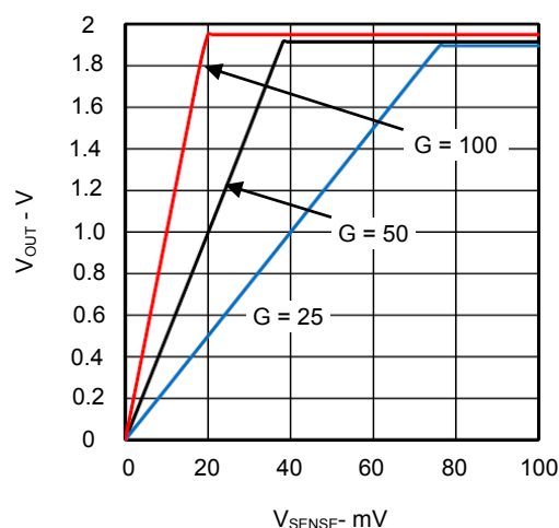
V_{OUT} vs V_{SENSE} @ Supply = 2V
