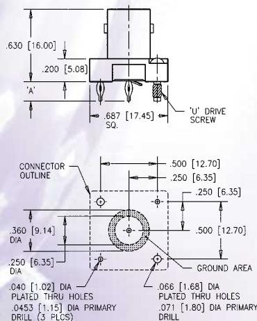
PCB LAYOUT (COMPONENT SIDE OF BOARD)
