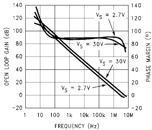
Gain and Phase
