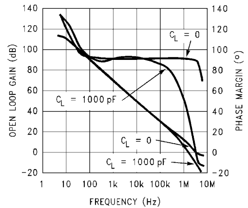
Gain and Phase, 2.7V Supply
