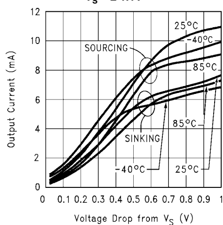
V_O vs. I_O V_S = \pm 1.1V
