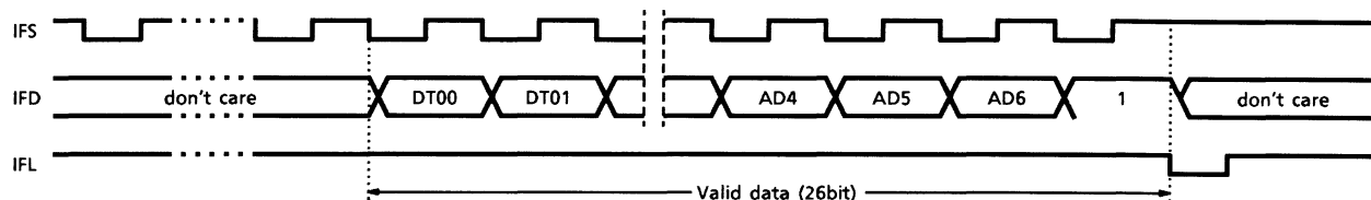
Figure 3 Example \mu -COM I/F
