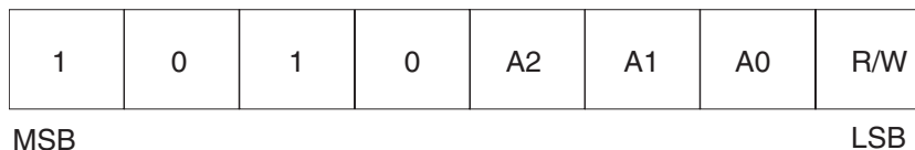
Figure 7-1. Device Address
