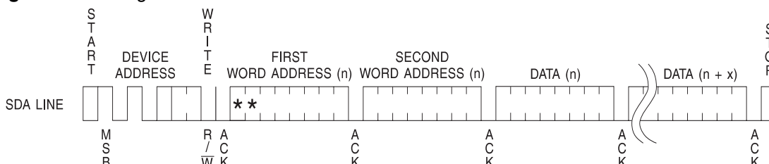
Figure 8-2. Page Write
