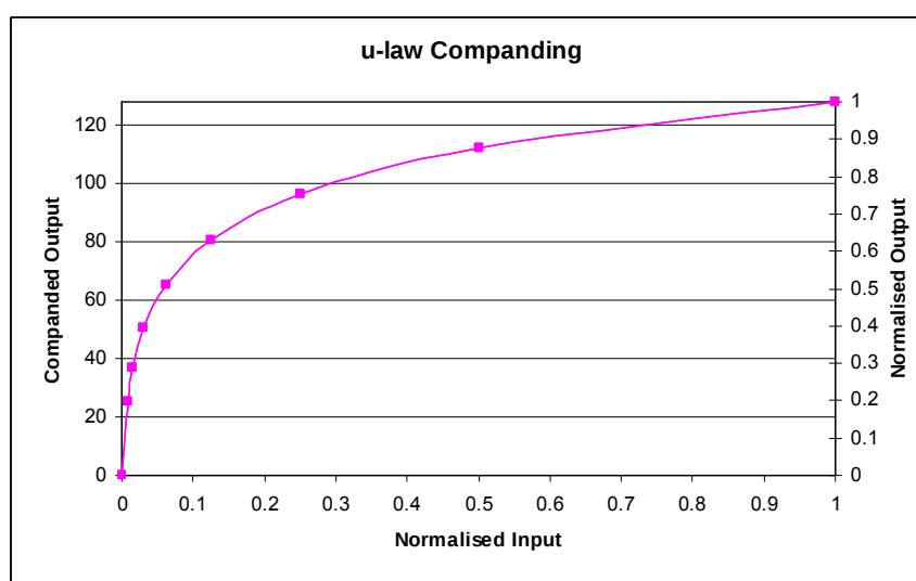
Figure 24 u-Law Companding
