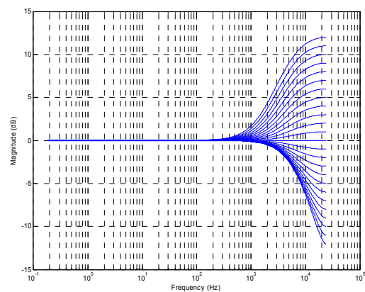
Figure 53 EQ Band 5 – High Frequency Shelf Filter Cut-offs
