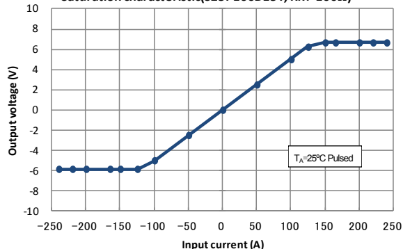
Saturation characteristic(S25P100D15Y, R_M=100\Omega )
