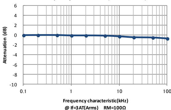
Frequency characteristic(S25P100D15Y)
