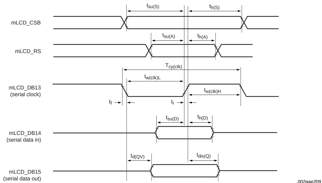
Fig 31. LCD timing (serial mode)
