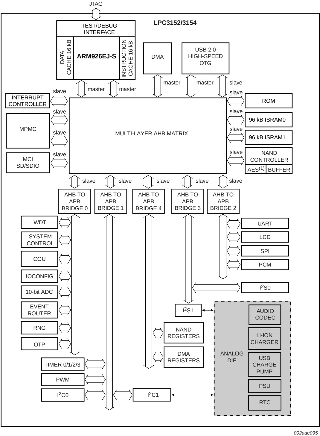
Fig 1. LPC3152/3154 block diagram
