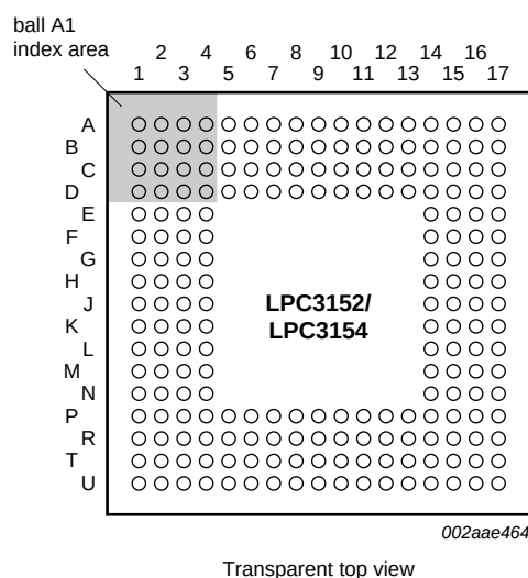
Fig 2. LPC3152/3154 pinning TFBGA208 package
