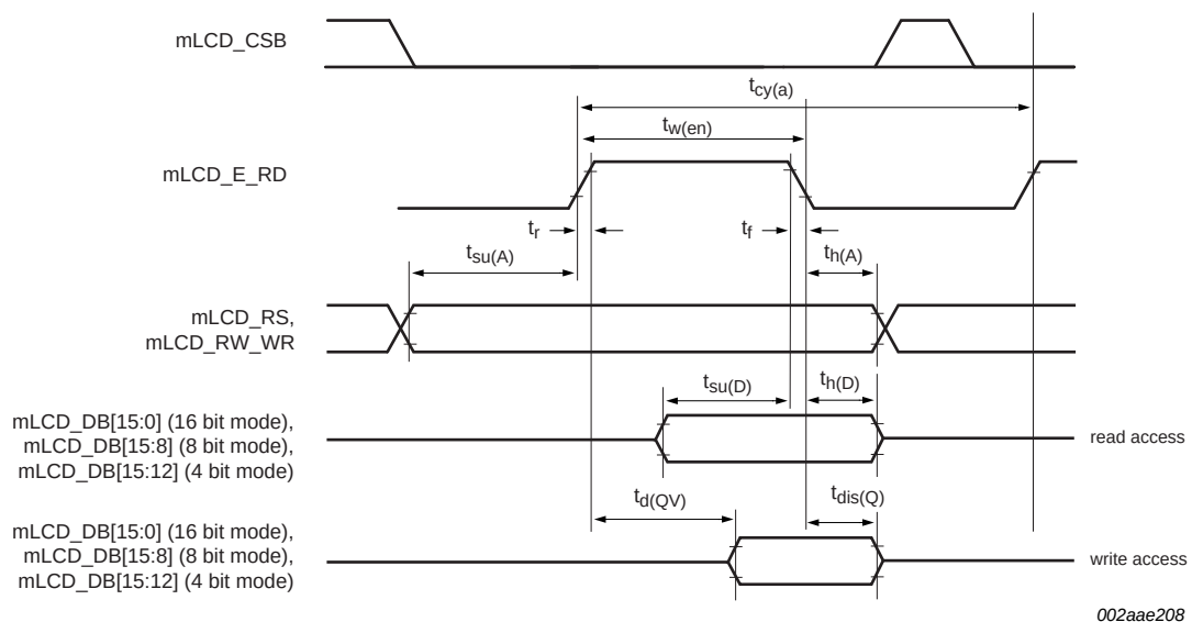
Fig 30. LCD timing (Motorola 6800 mode)
