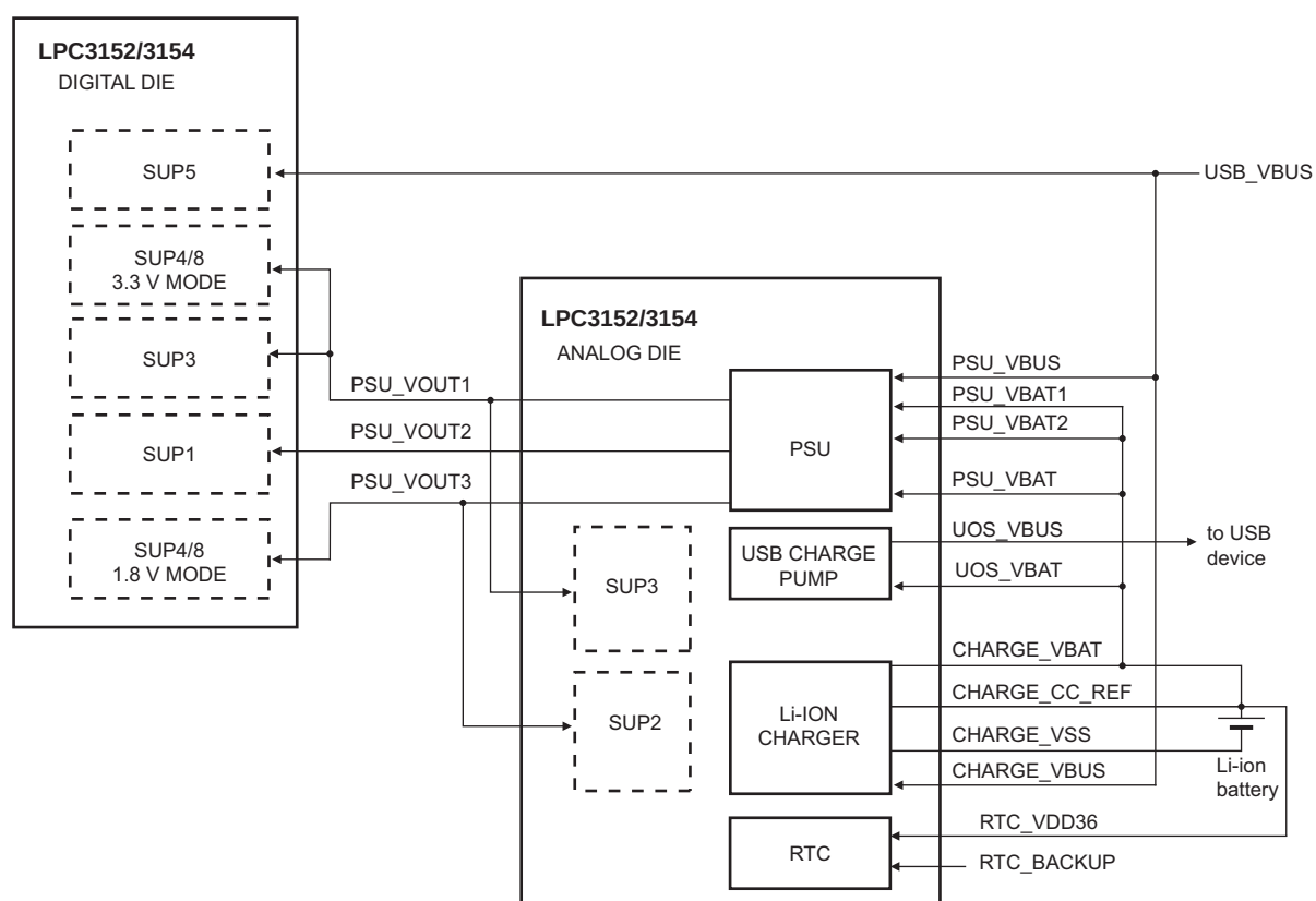
Fig 13. LPC3152/3154 supply voltages of the analog and digital die
