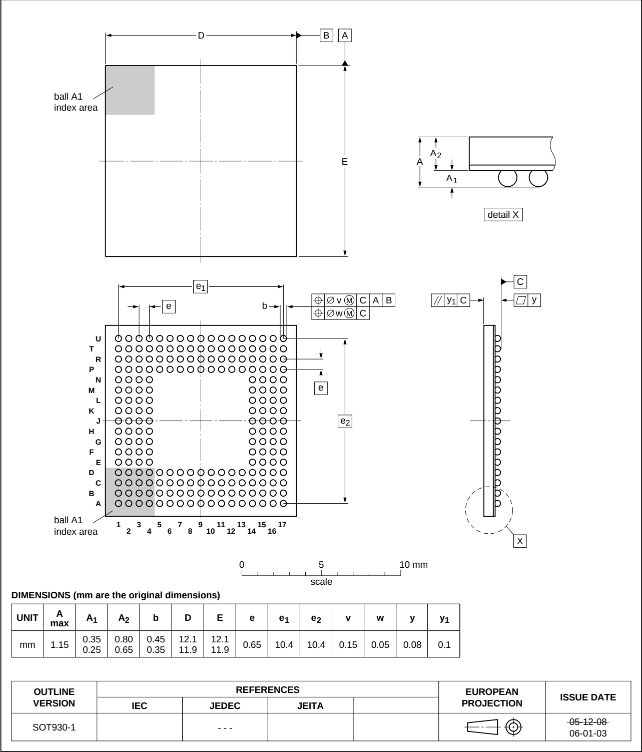
Fig 42. LPC3152/3154 TFBGA208 package outline
