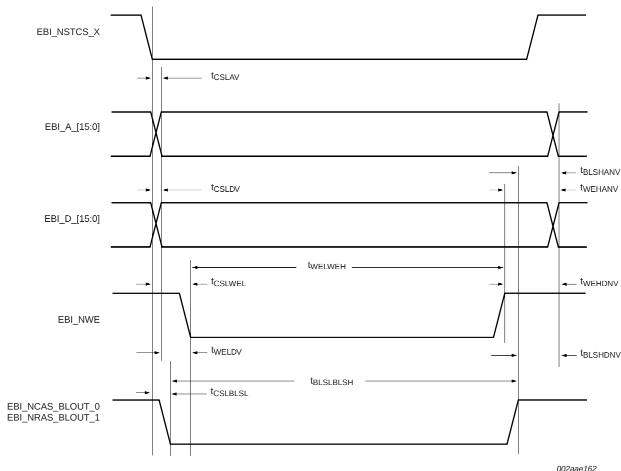
Fig 33. External memory write access to static memory
