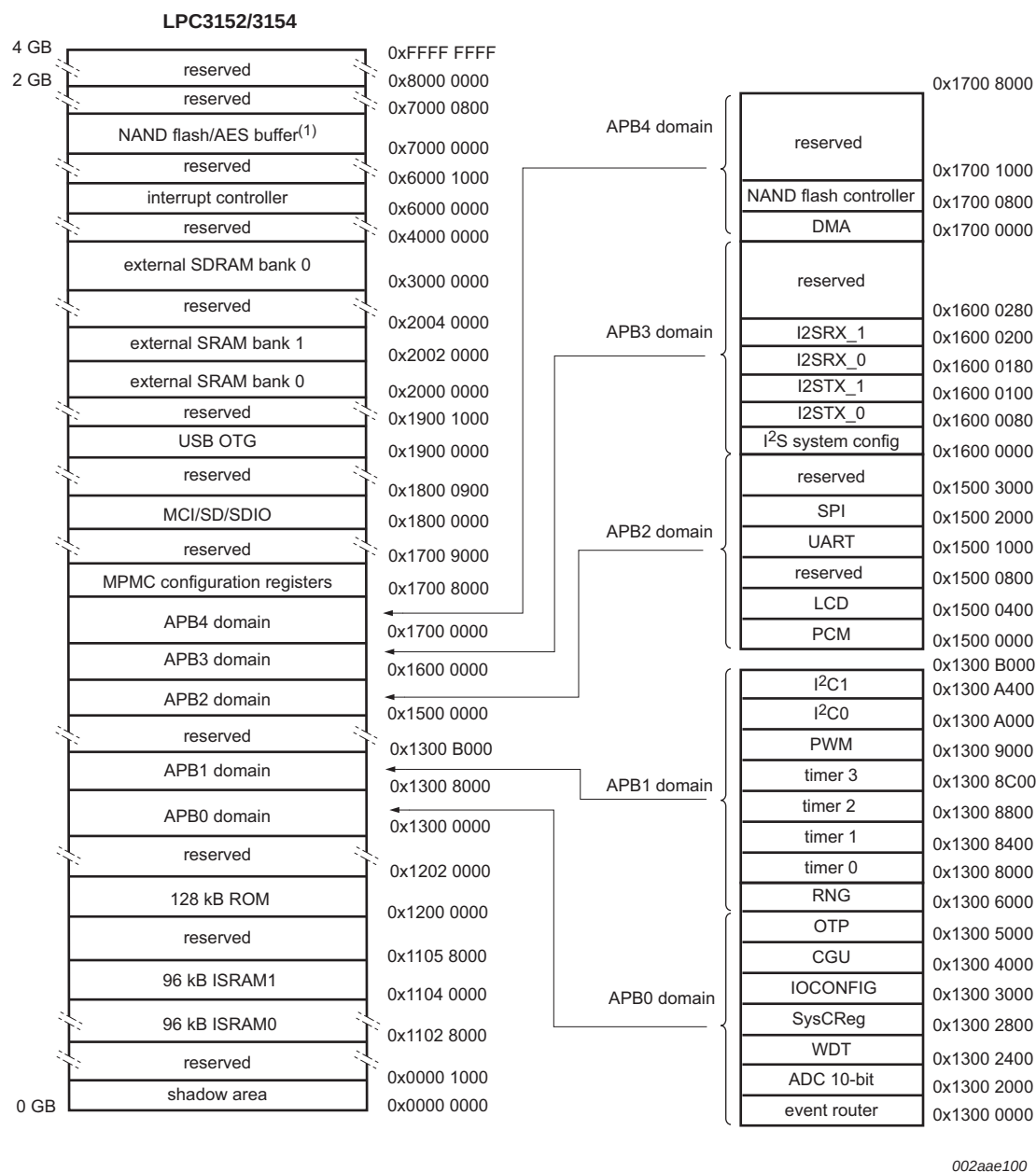
Fig 3. LPC3152/3154 memory map
