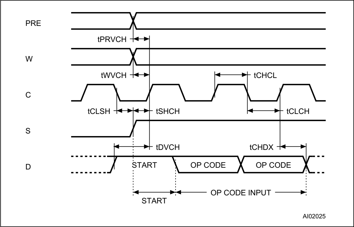
Figure 9. Synchronous timing (start and op-code input)
