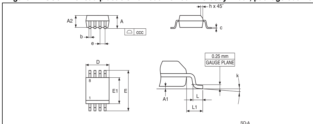
Figure 12. SO8N – 8-lead plastic small outline 150 mils body width, package outline
