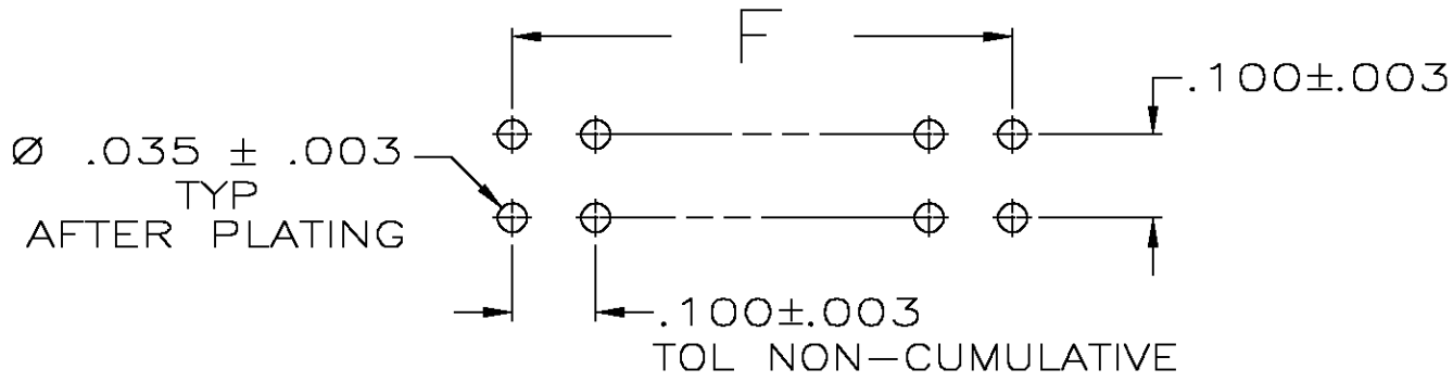
RECOMMENDED HOLE LAYOUT
