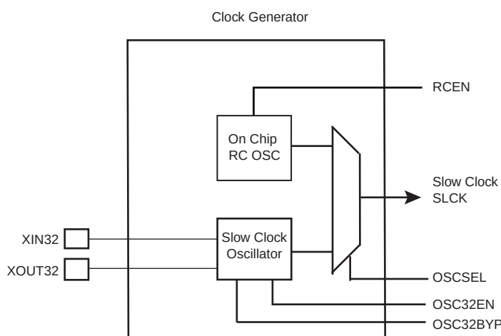
Figure 8-3. Slow Clock
