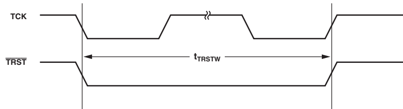
Figure 29. JTAG Port Reset Timing
