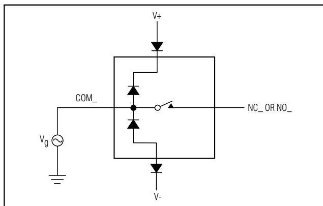
Figure 6. Overvoltage Protection Using Blocking Diodes
