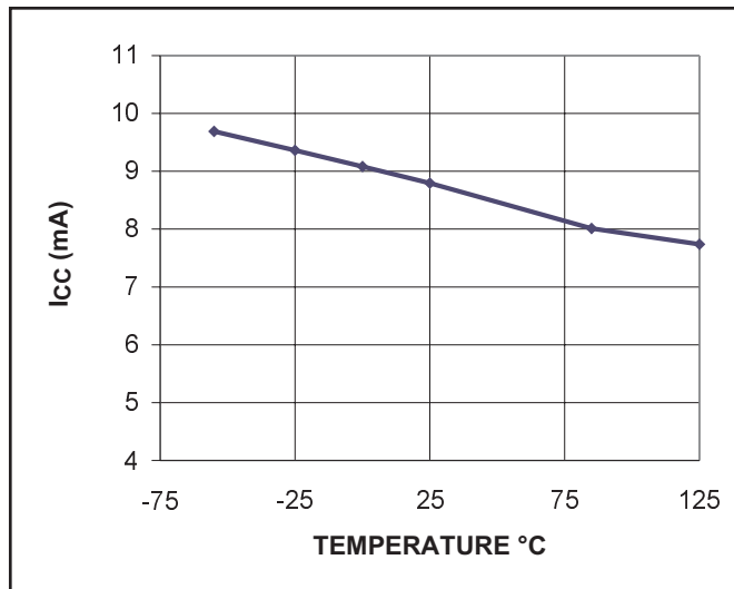
Figure 1. Supply Current
