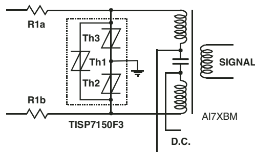
Figure 22. ISDN Protection
