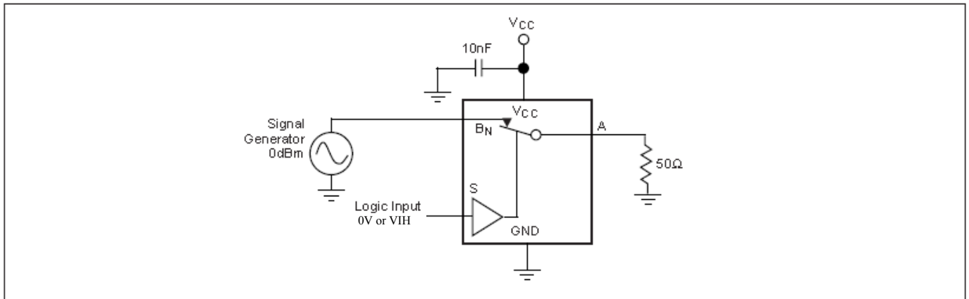
Figure 8. Bandwidth
