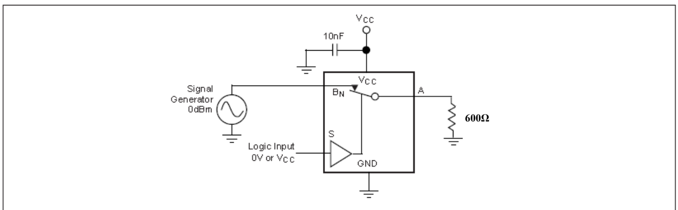
Figure 9. Harmonic Distortion
