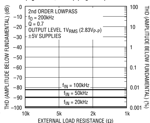
Distortion vs External Load Resistance and Frequency ( V_S = \pm 5V , 25°C) (Figure 8)
