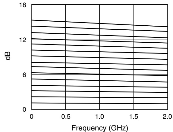
Attenuation vs. Frequency (All States)
