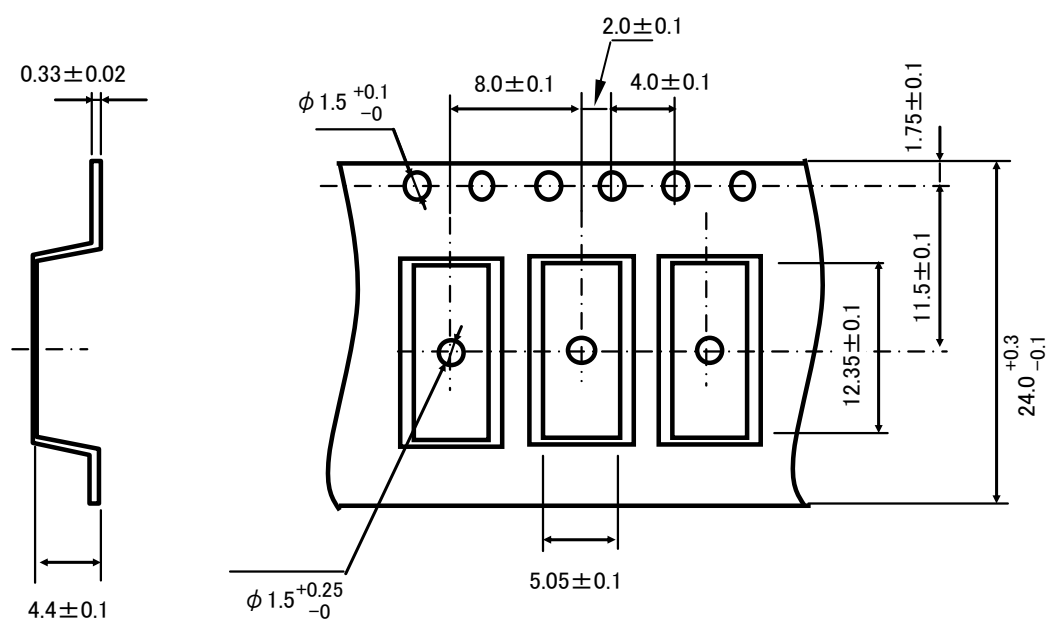
Figure 3 Tape Forms
