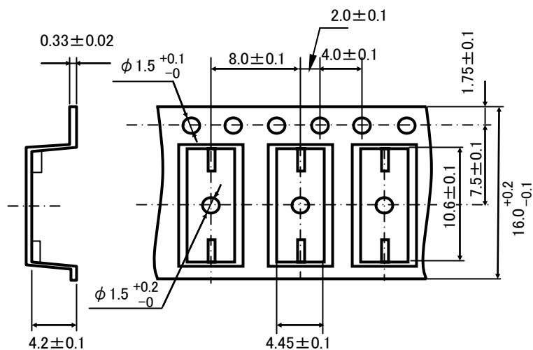
Figure 2 Tape Forms
