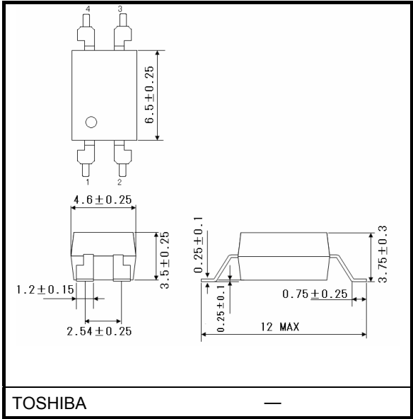
TLP781F(LF7)
