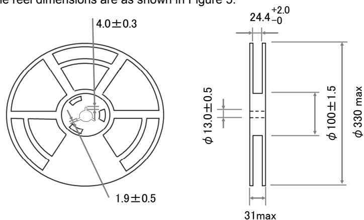
Figure 5 Reel Forms
