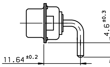
VIEW WITH POWERS CONTACTS
