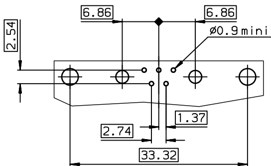
LAYOUT DIMENSIONS (after plating) CONNECTOR SIDE VIEW
