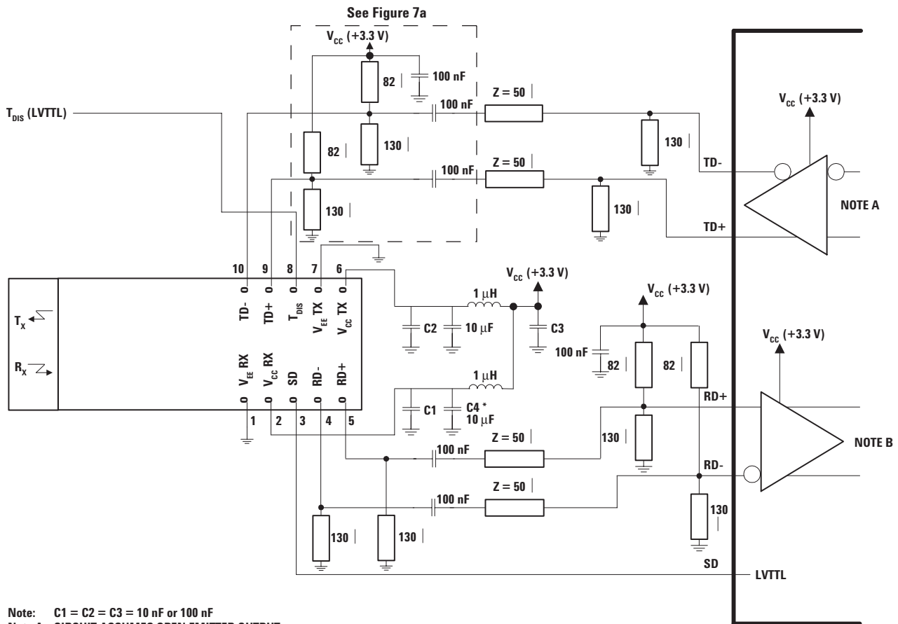
Figure 8. Recommended Interface Circuit (HFCT-5951TLZ/TGZ/ATLZ/ATGZ)
