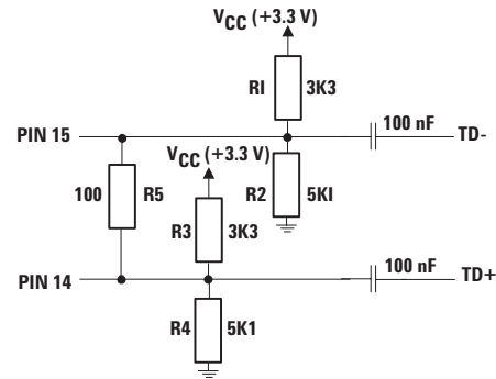
Figure 7b. Low current dc biasing scheme
