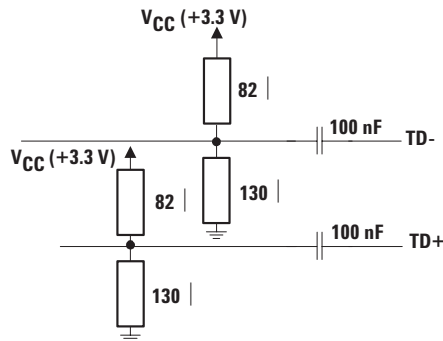
Figure 7a. LVPECL termination and biasing scheme
