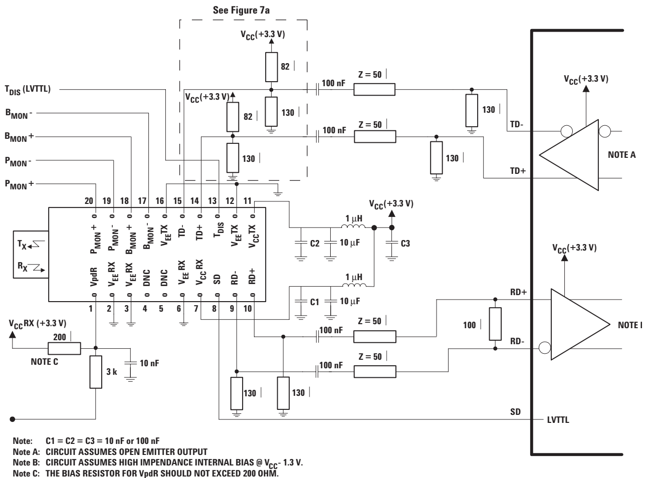
Figure 7. Recommended Interface Circuit (HFCT-5952TLZ/TGZ/ATLZ/ATGZ)
