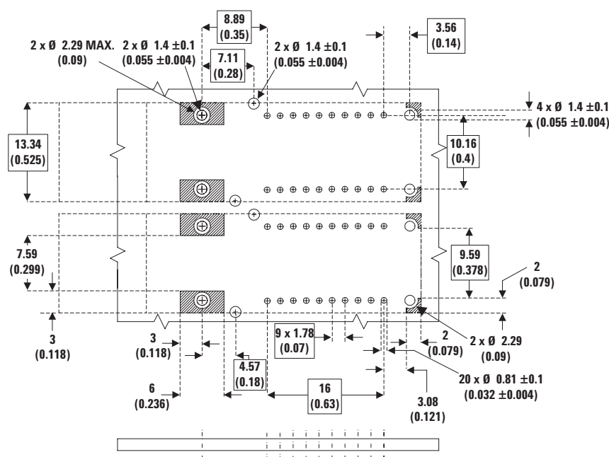
Figure 9. Recommended Board Layout Hole Pattern
