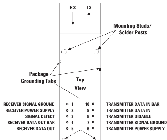
Figure 6. Pin Out Diagram (Top View)
