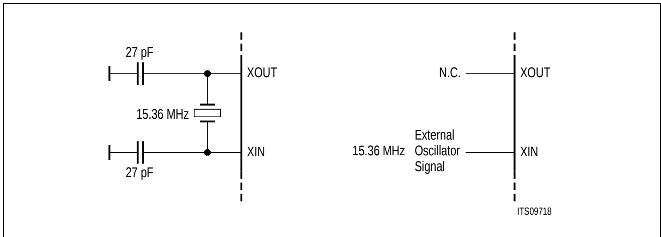
Figure 45 Crystal Oscillator or External Clock Source
