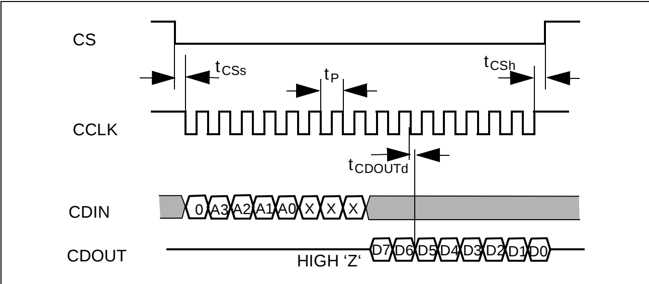
Figure 59 Serial μP Interface Mode Read
