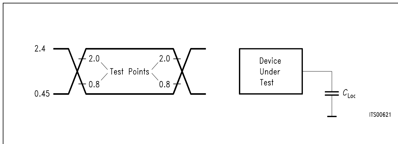
Figure 50 Input/Output Waveform for AC Tests
