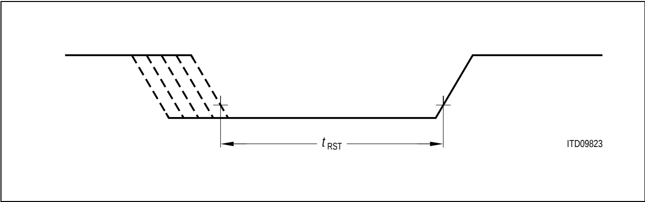
Figure 63 Reset Signal
