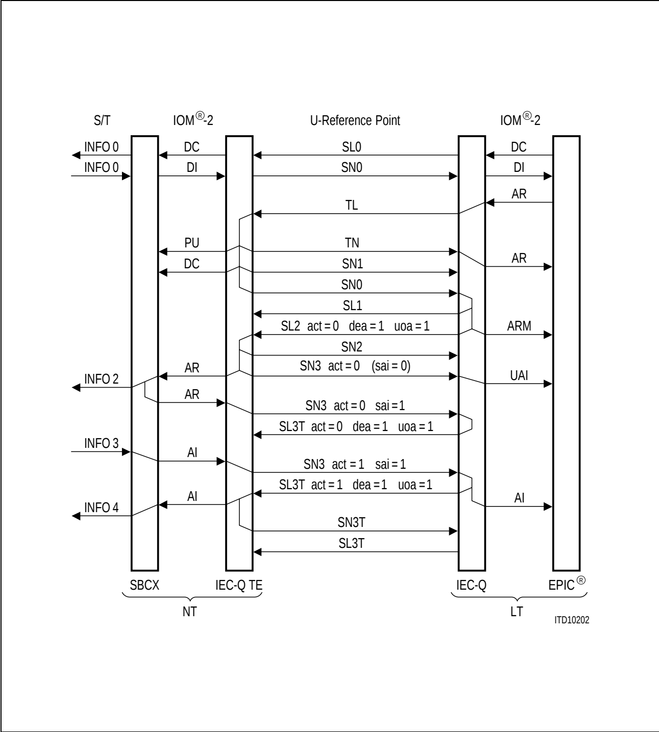
Figure 35 Complete Activation Initiated by LT
