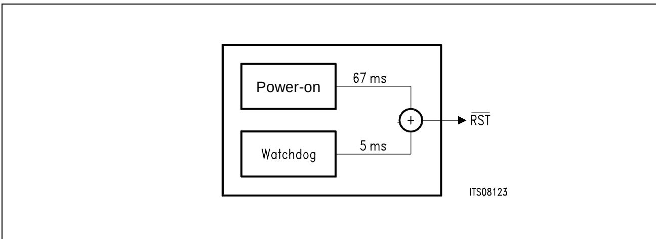
Figure 32 Reset Sources
