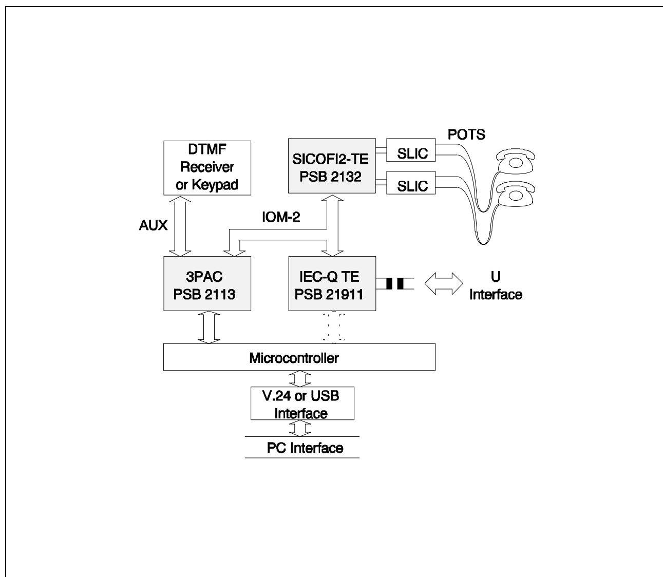
Figure 6 ISDN Stand-Alone Terminal with POTS Interface
