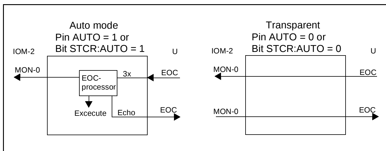
Figure 20 EOC-Processor: Auto Mode, Transparent Mode
