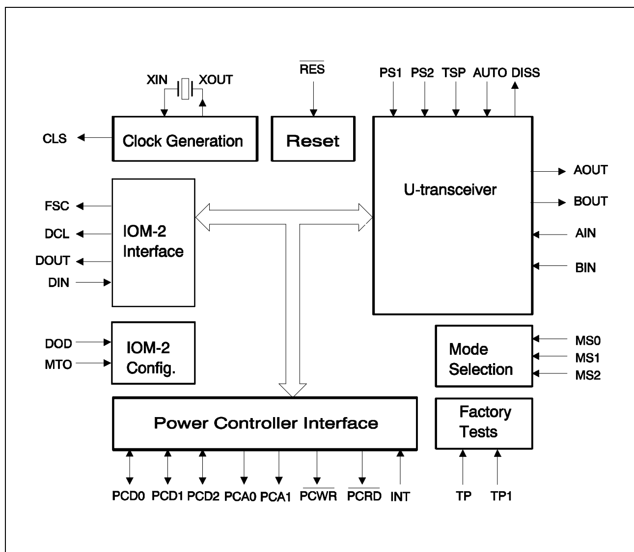
Figure 10 IEC-Q TE Device Architecture (Stand-Alone Mode)
