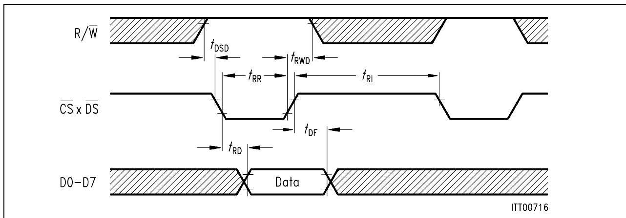
Figure 55 Motorola Read Timing
