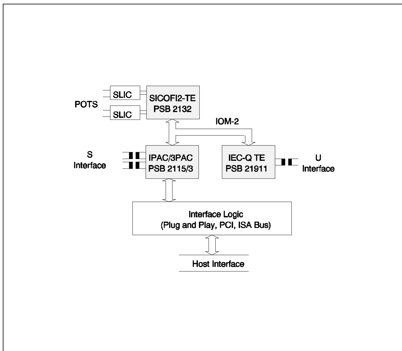
Figure 5 ISDN PC Adapter Card
