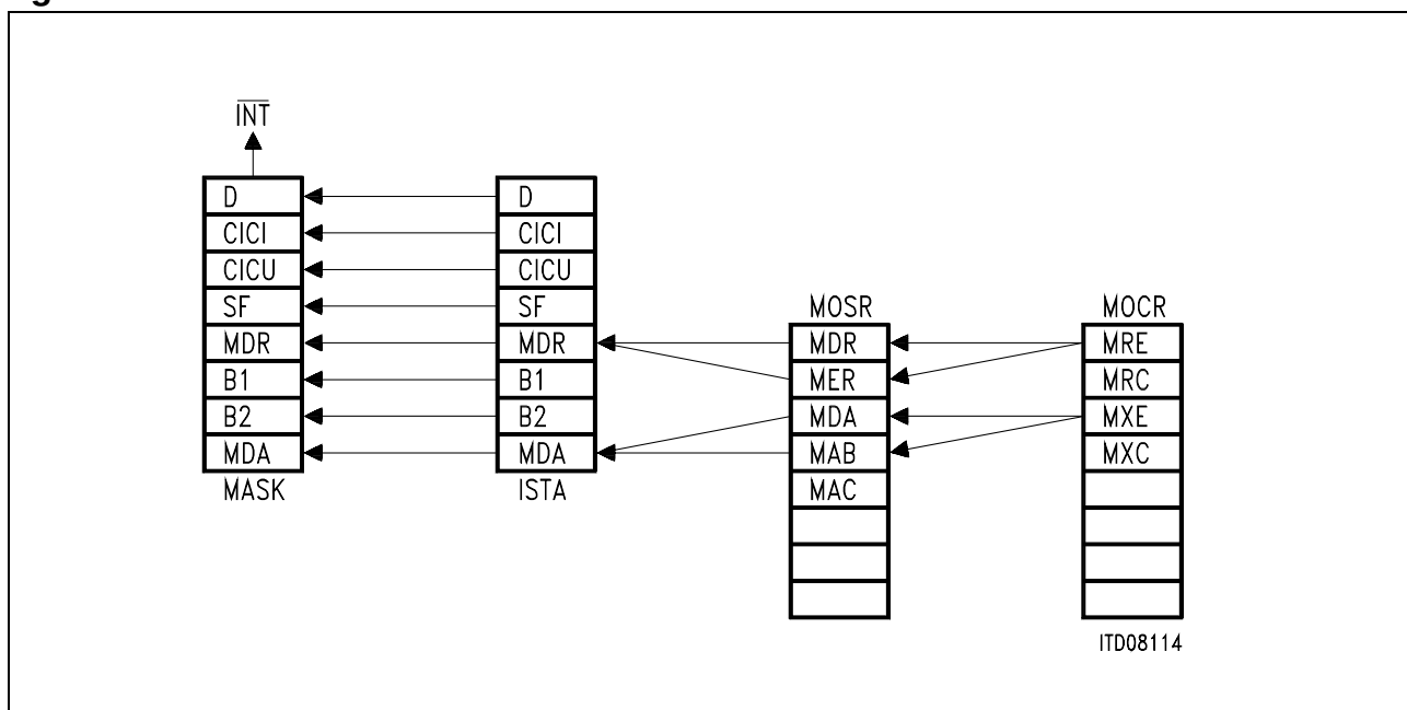
Figure 46 Interrupt Structure
