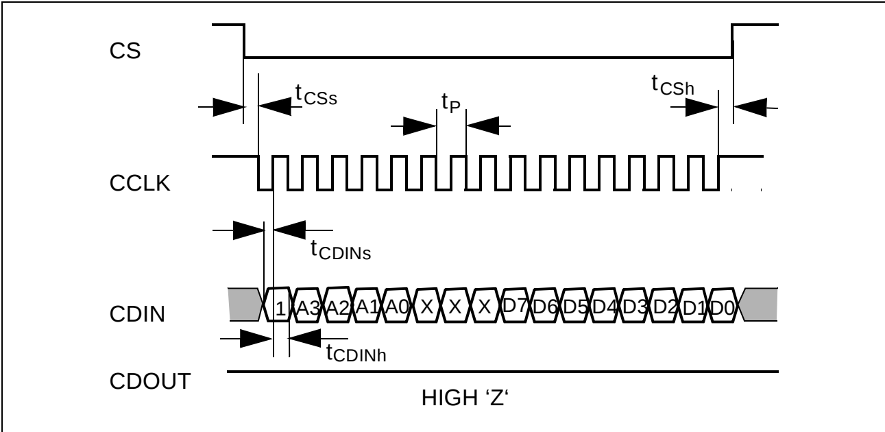
Figure 58 Serial μP Interface Mode Write
