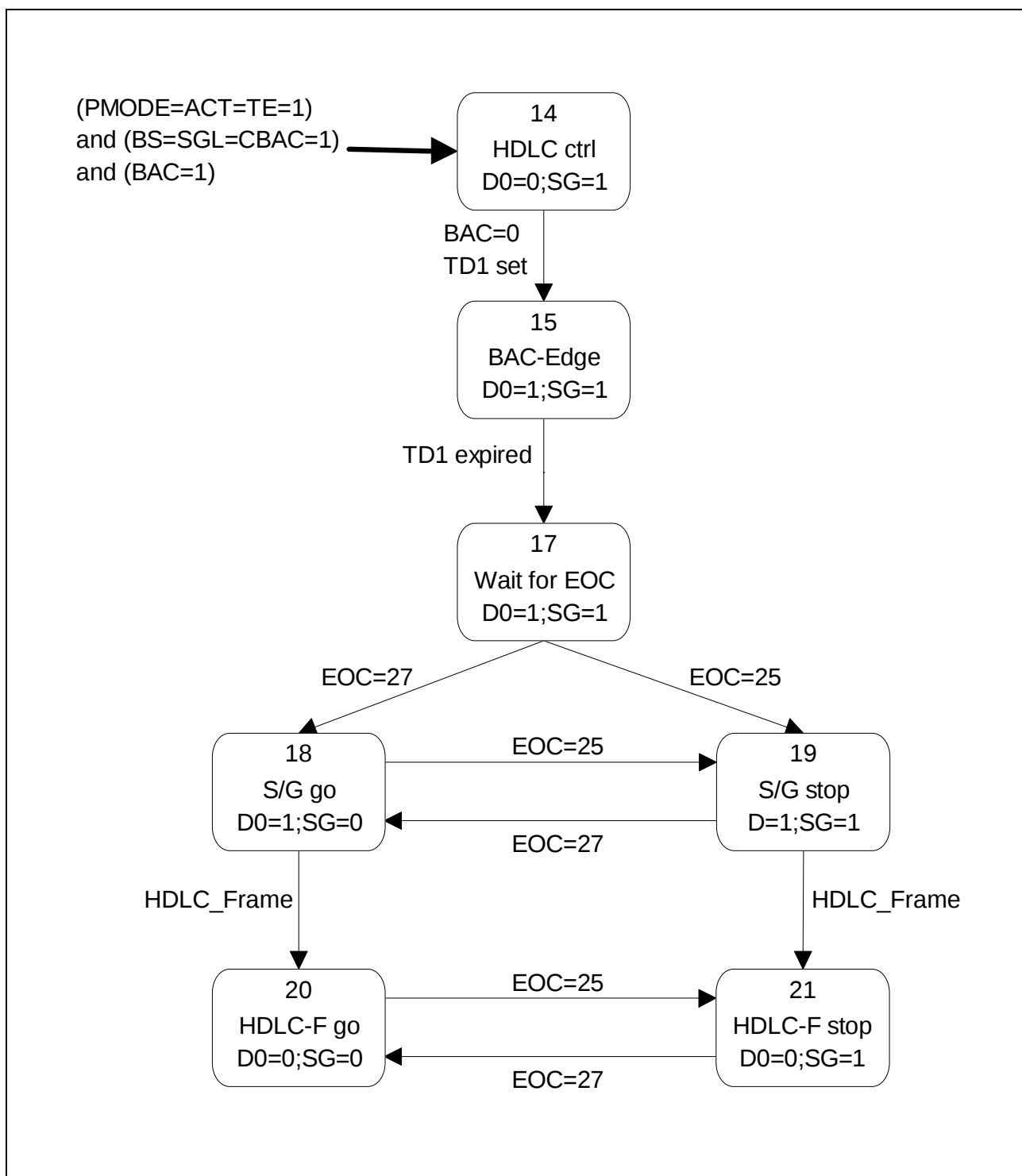
Figure 67 State machine (part 3)
