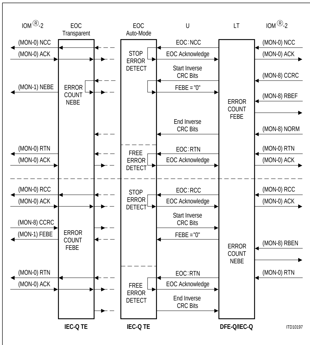
Figure 18 Block Error Counter Test
