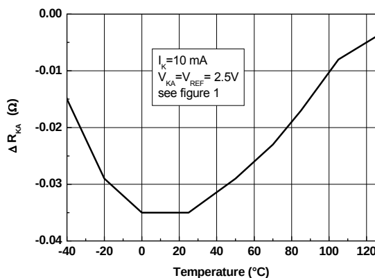
Figure 17. Drift of R_{KA} vs. temperature
