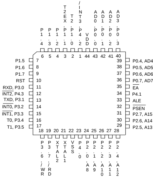
44-Pin PLCC
