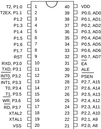
40-Pin DIP
