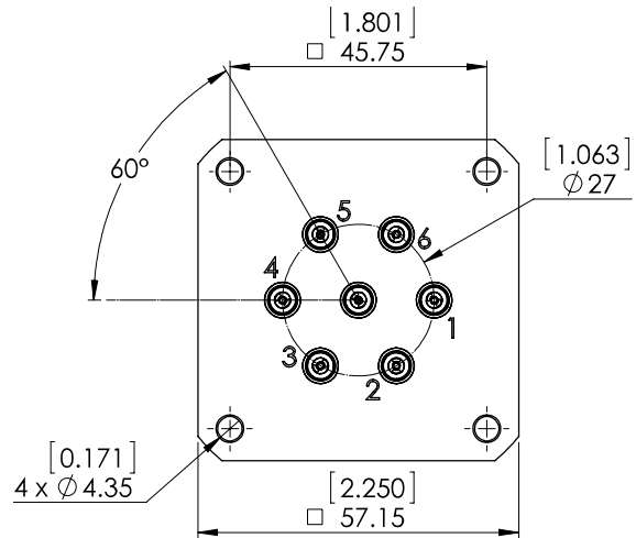
SMA 2.9 Connectors
