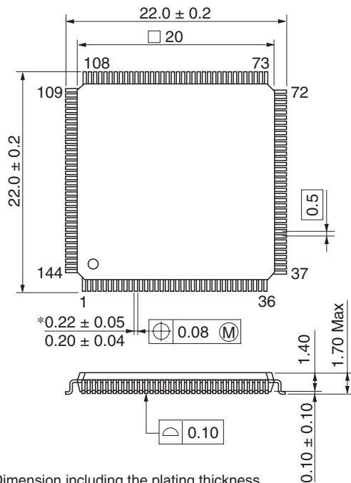
Figure E.2 FP-144F
