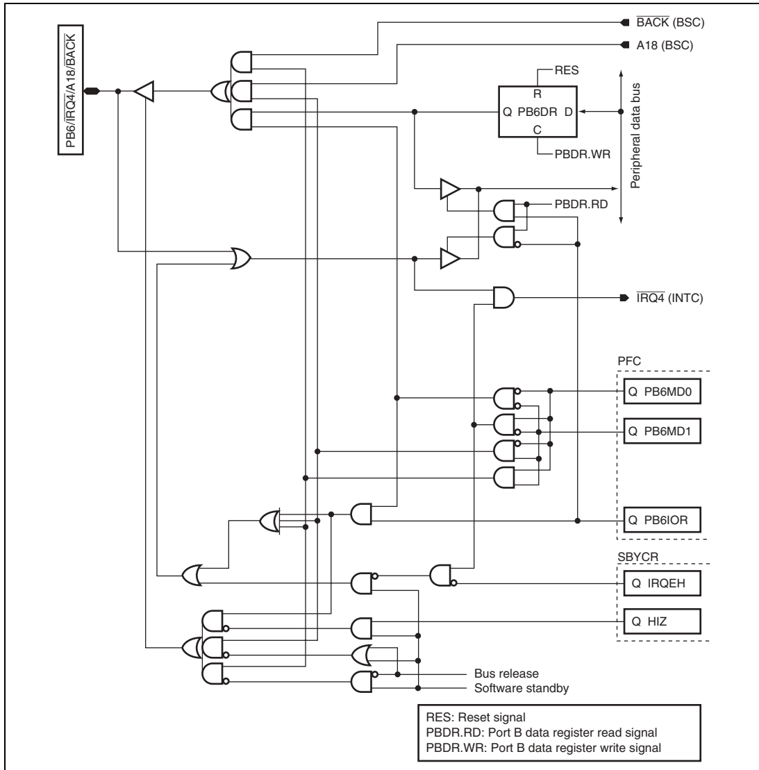
Figure D.18 PB6/\overline{IRQ4}/A18/\overline{BACK}
