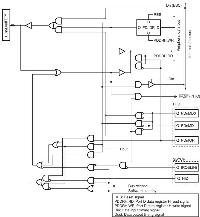
Figure D.27 PDn/Dn/ \overline{\text{IRQm}}
