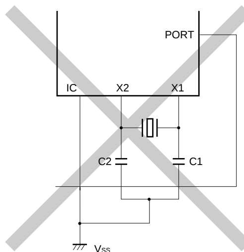
(b) Crossed signal line
