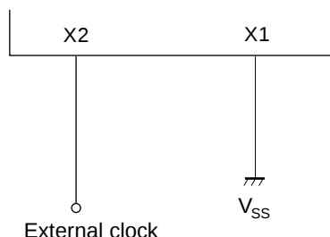
Figure 2-2: External Clock Input
