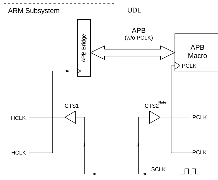
Figure 2-8: Clock Structure
