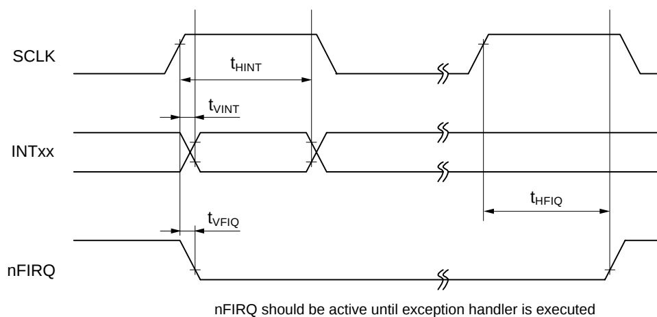
Figure 2-19: Interrupt Cycle
