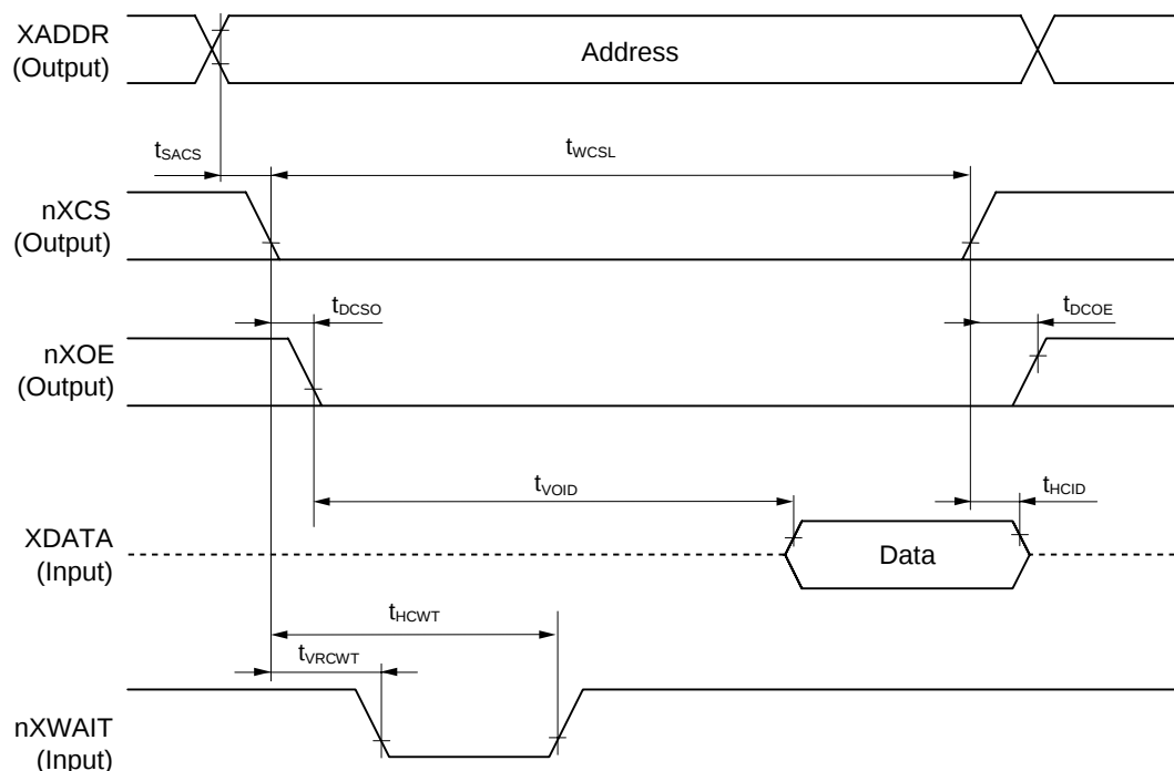
Figure 2-11: External Memory Bus Single Read Cycle
