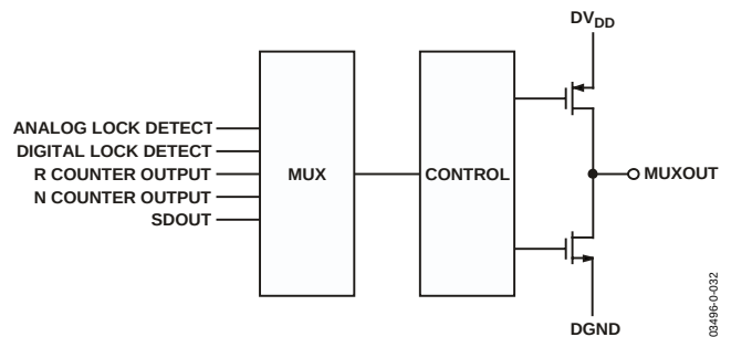
Figure 32. MUXOUT Circuit
