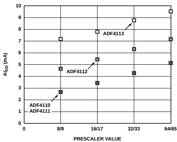
Figure 25. A_{IDD} vs. Prescaler Value
