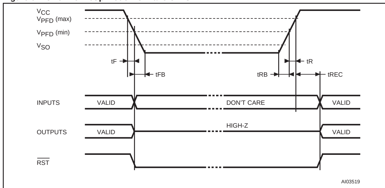
Figure 9. Power Down/Up Mode AC Waveforms
