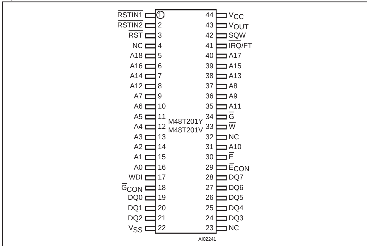
Figure 3. SOIC Connections
