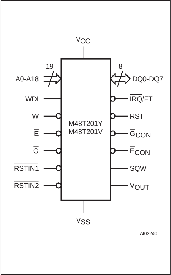
Figure 2. Logic Diagram
