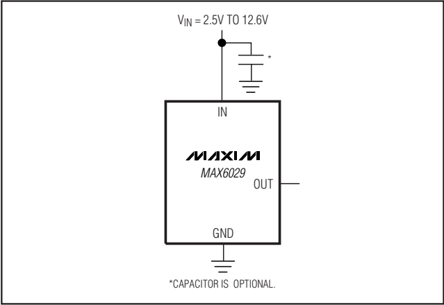
Typical Operating Circuit
