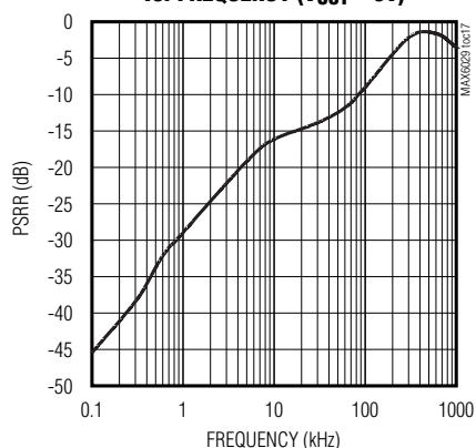
POWER-SUPPLY REJECTION RATIO vs. FREQUENCY ( V_{OUT} = 5V )
