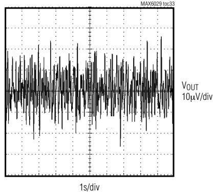
0.1Hz TO 10Hz OUTPUT NOISE ( V_{OUT} = 3V )
