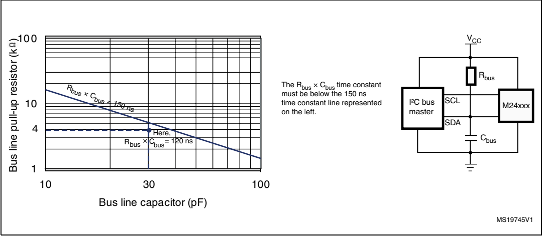
Figure 14. Maximum R_{bus} value versus bus parasitic capacitance C_{bus} ) for an I2C bus at maximum frequency f_C = 1 \text{ MHz}
