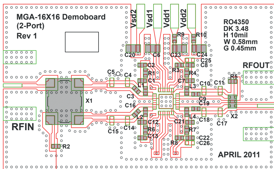
Figure 18. Balanced Amplifier Demo Board Layout Diagram
