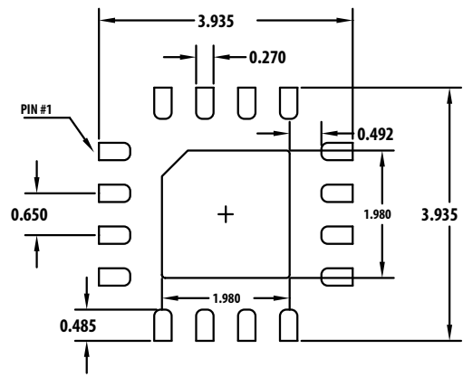
Stencil Opening
