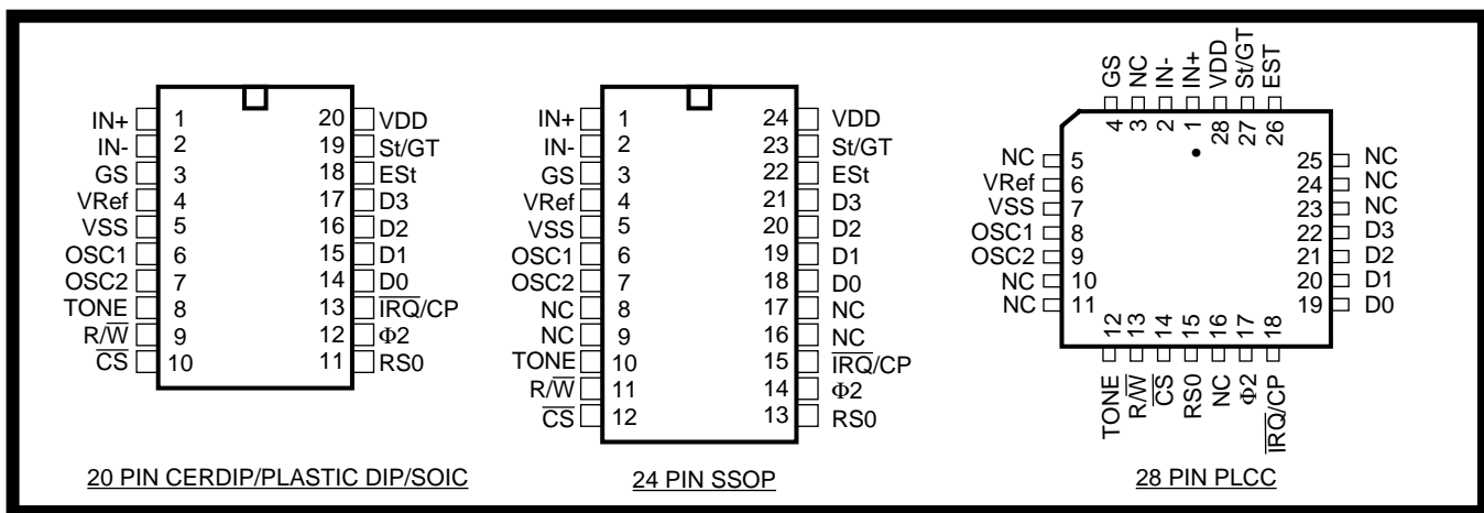
Figure 2 - Pin Connections
