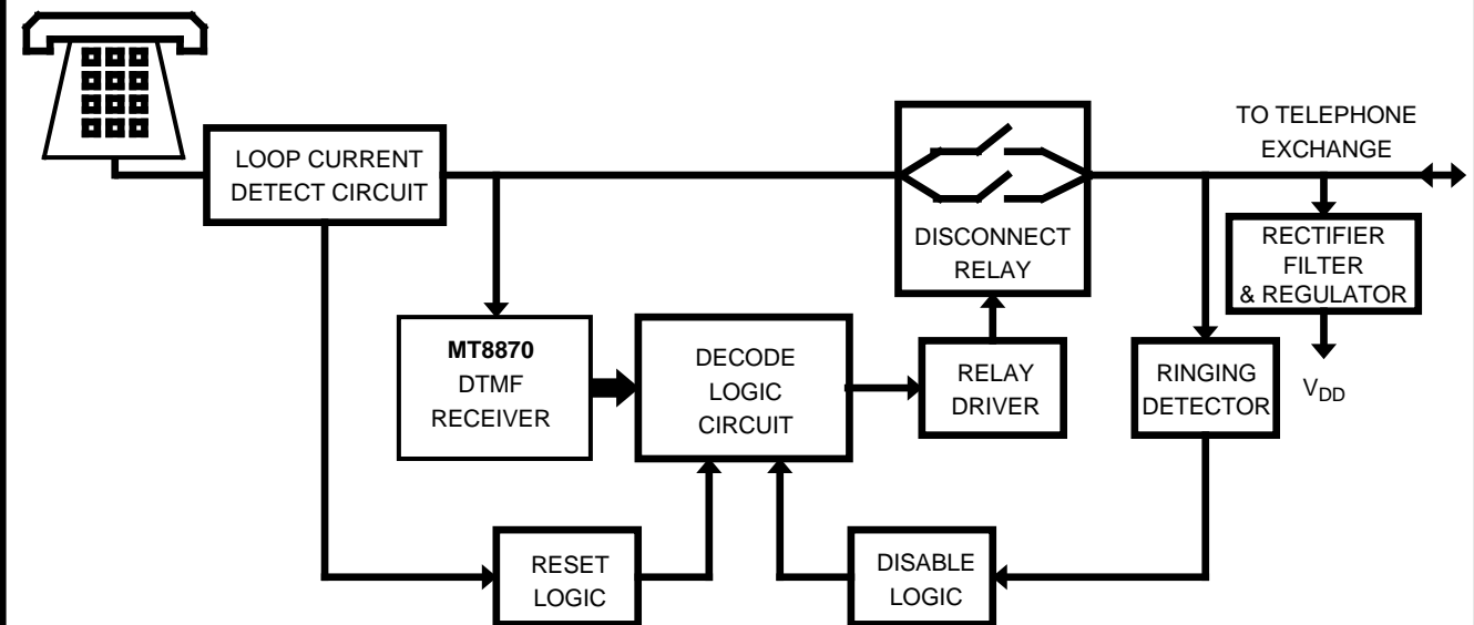
a) Block diagram of a toll call restrictor. This could be implemented on a small pc board and installed in a telephone to disallow long distance calling.
