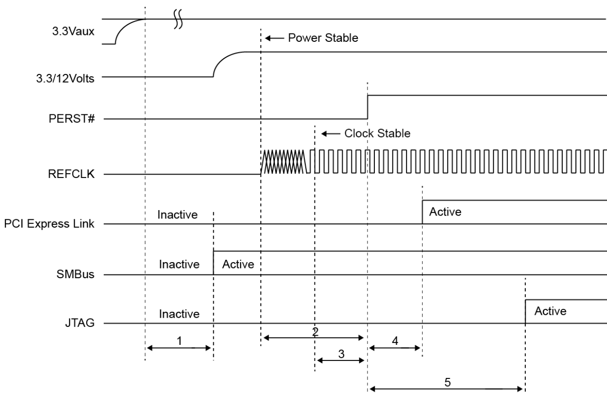
Figure 14-3 Initial Power-up
