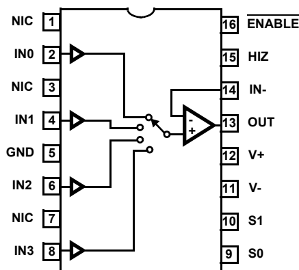
ISL59441 (16 LD QSOP) TOP VIEW
