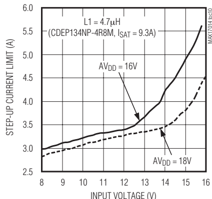
STEP-UP REGULATOR CURRENT LIMIT vs. INPUT VOLTAGE
