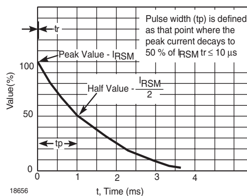
Figure 2. Pulse Waveform
