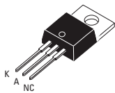
TO-220AB Isolated (CRNA25...L3)
