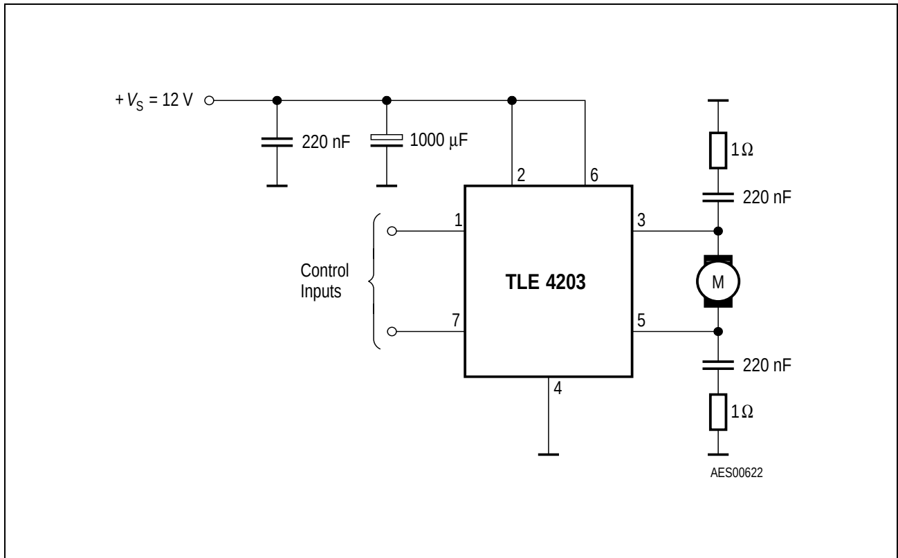
Figure 5 Application Circuit
