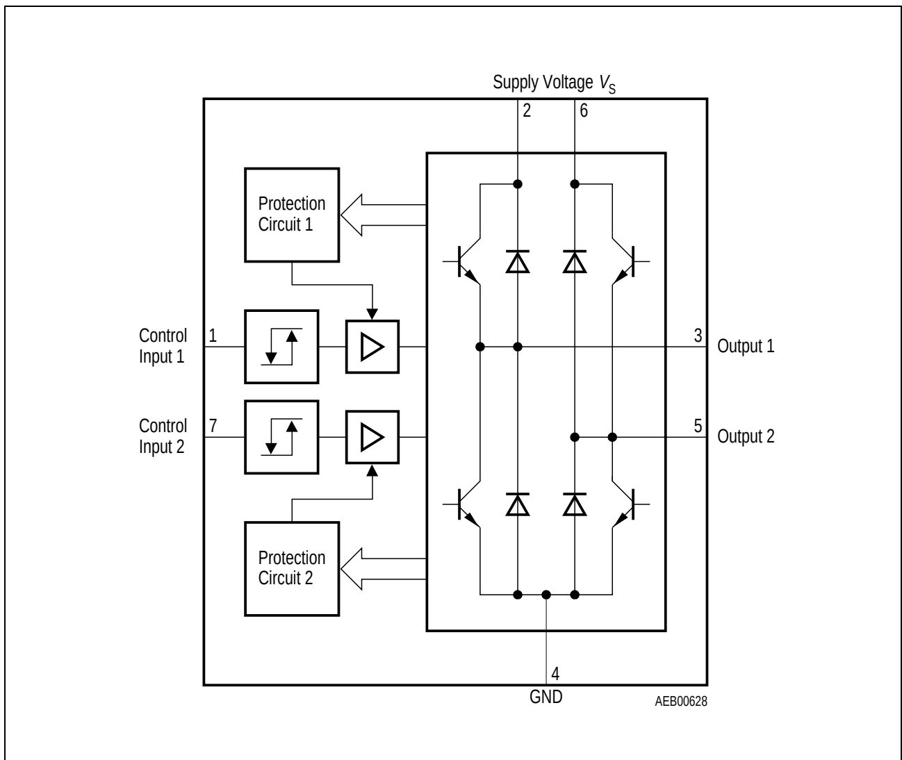
Figure 2 Block Diagram
